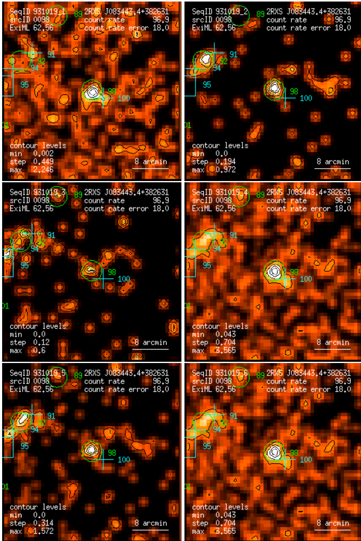
Figure 98: RASS 931019: detection 0098: band rate images, Gaussian filter: (1) PSPC channels 11 – 41, (2) 52 – 90, (3) 91 – 201, (4) 11 – 235, (5) 52 – 201, (6) 11 – 201. Broad band rates in counts/ks. Band rate contour levels in counts/ks/arcmin 2 .
