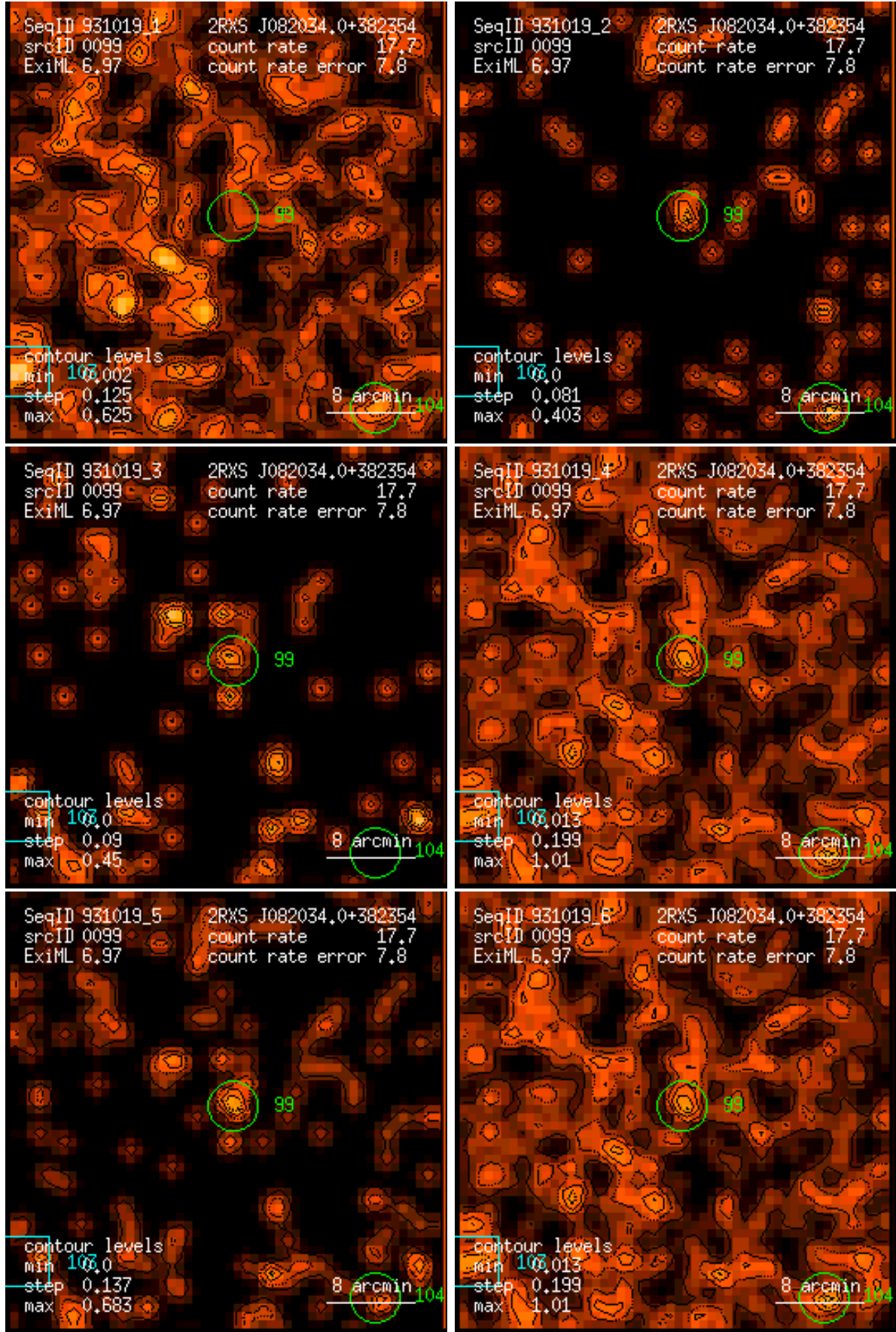
Figure 99: RASS 931019: detection 0099: band rate images, Gaussian filter: (1) PSPC channels 11 – 41, (2) 52 – 90, (3) 91 – 201, (4) 11 – 235, (5) 52 – 201, (6) 11 – 201. Broad band rates in counts/ks. Band rate contour levels in counts/ks/arcmin 2 .
