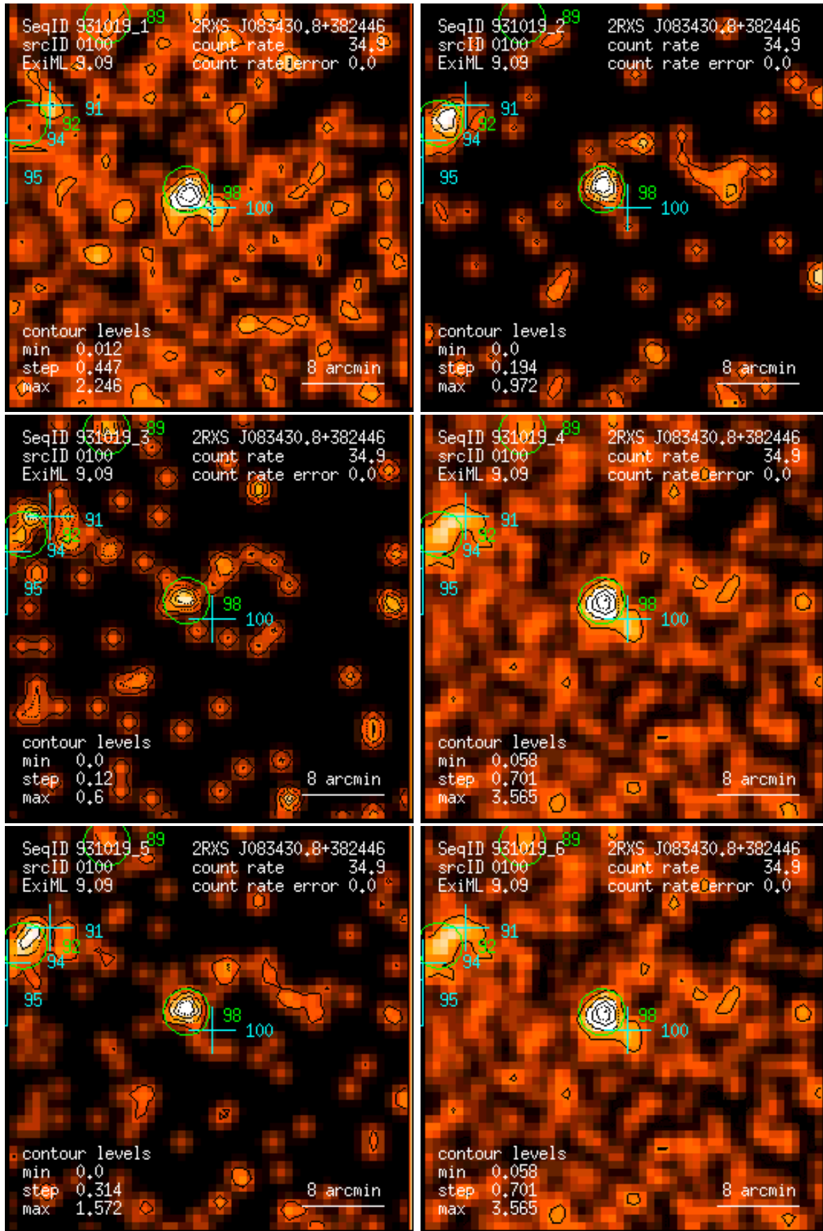
Figure 100: RASS 931019: detection 0100: band rate images, Gaussian filter: (1) PSPC channels 11 – 41, (2) 52 – 90, (3) 91 – 201, (4) 11 – 235, (5) 52 – 201, (6) 11 – 201. Broad band rates in counts/ks. Band rate contour levels in counts/ks/arcmin 2 .
