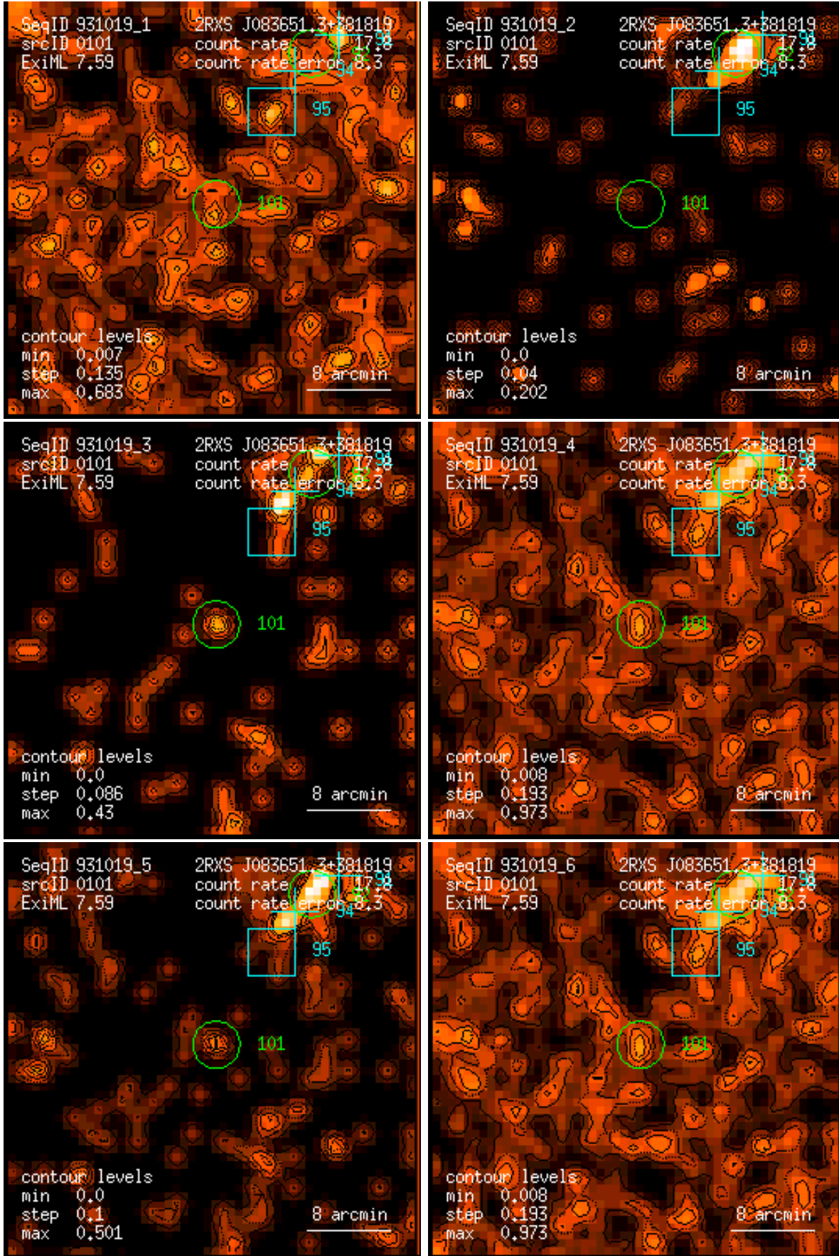
Figure 101: RASS 931019: detection 0101: band rate images, Gaussian filter: (1) PSPC channels 11 – 41, (2) 52 – 90, (3) 91 – 201, (4) 11 – 235, (5) 52 – 201, (6) 11 – 201. Broad band rates in counts/ks. Band rate contour levels in counts/ks/arcmin 2 .
