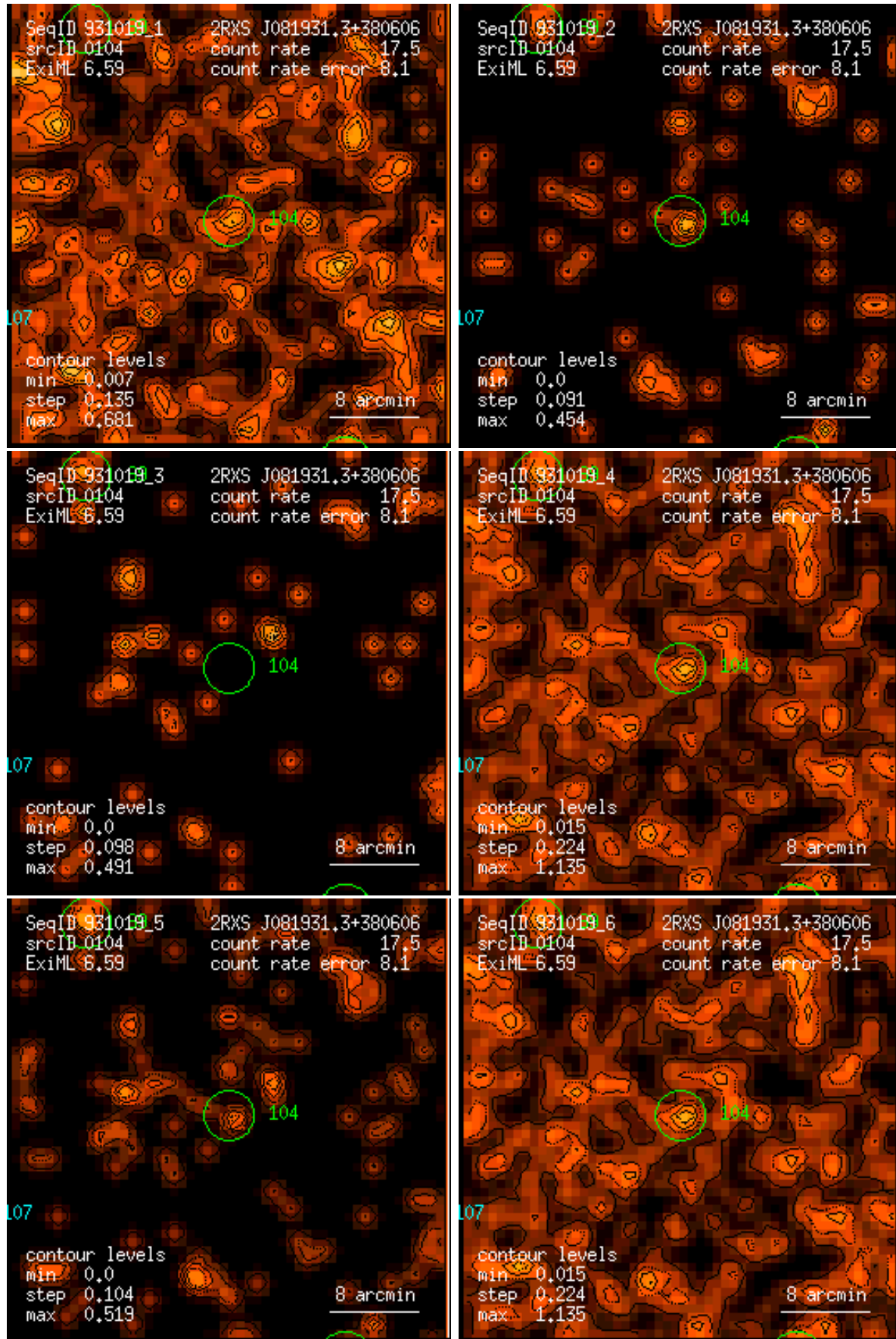
Figure 104: RASS 931019: detection 0104: band rate images, Gaussian filter: (1) PSPC channels 11 – 41, (2) 52 – 90, (3) 91 – 201, (4) 11 – 235, (5) 52 – 201, (6) 11 – 201. Broad band rates in counts/ks. Band rate contour levels in counts/ks/arcmin 2 .
