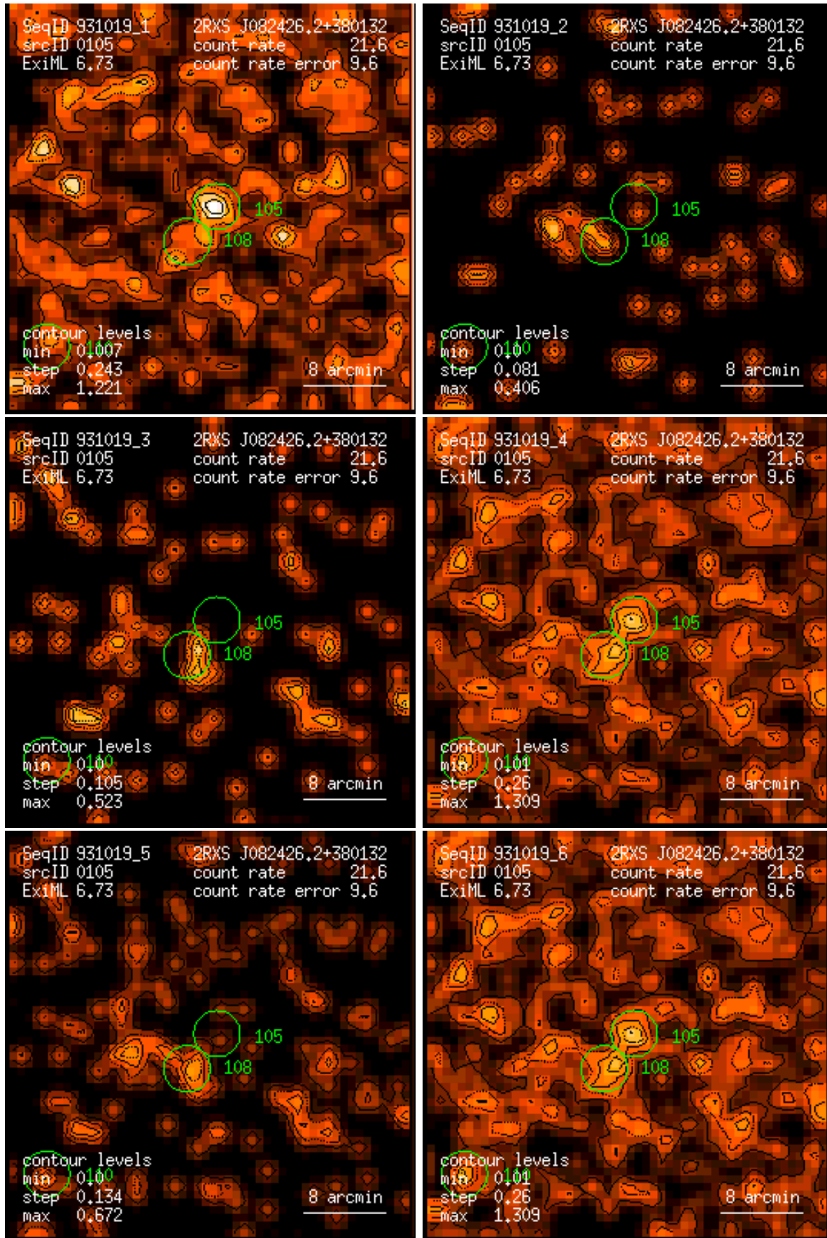
Figure 105: RASS 931019: detection 0105: band rate images, Gaussian filter: (1) PSPC channels 11 – 41, (2) 52 – 90, (3) 91 – 201, (4) 11 – 235, (5) 52 – 201, (6) 11 – 201. Broad band rates in counts/ks. Band rate contour levels in counts/ks/arcmin 2 .
