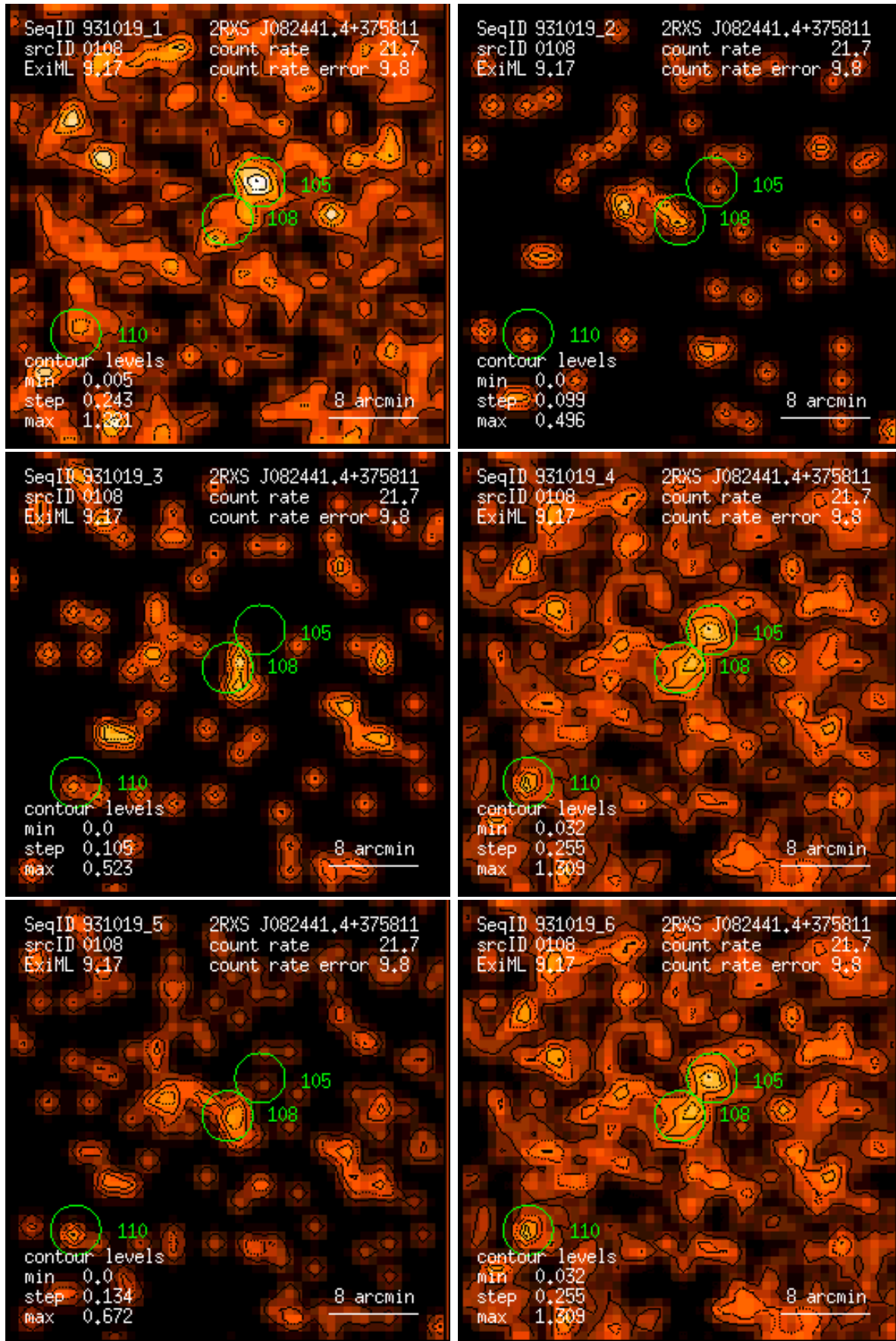
Figure 108: RASS 931019: detection 0108: band rate images, Gaussian filter: (1) PSPC channels 11 – 41, (2) 52 – 90, (3) 91 – 201, (4) 11 – 235, (5) 52 – 201, (6) 11 – 201. Broad band rates in counts/ks. Band rate contour levels in counts/ks/arcmin 2 .
