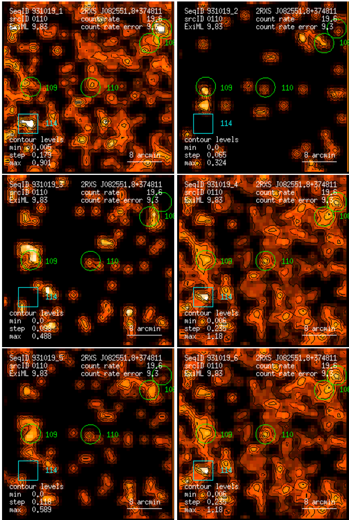
Figure 110: RASS 931019: detection 0110: band rate images, Gaussian filter: (1) PSPC channels 11 – 41, (2) 52 – 90, (3) 91 – 201, (4) 11 – 235, (5) 52 – 201, (6) 11 – 201. Broad band rates in counts/ks. Band rate contour levels in counts/ks/arcmin 2 .
