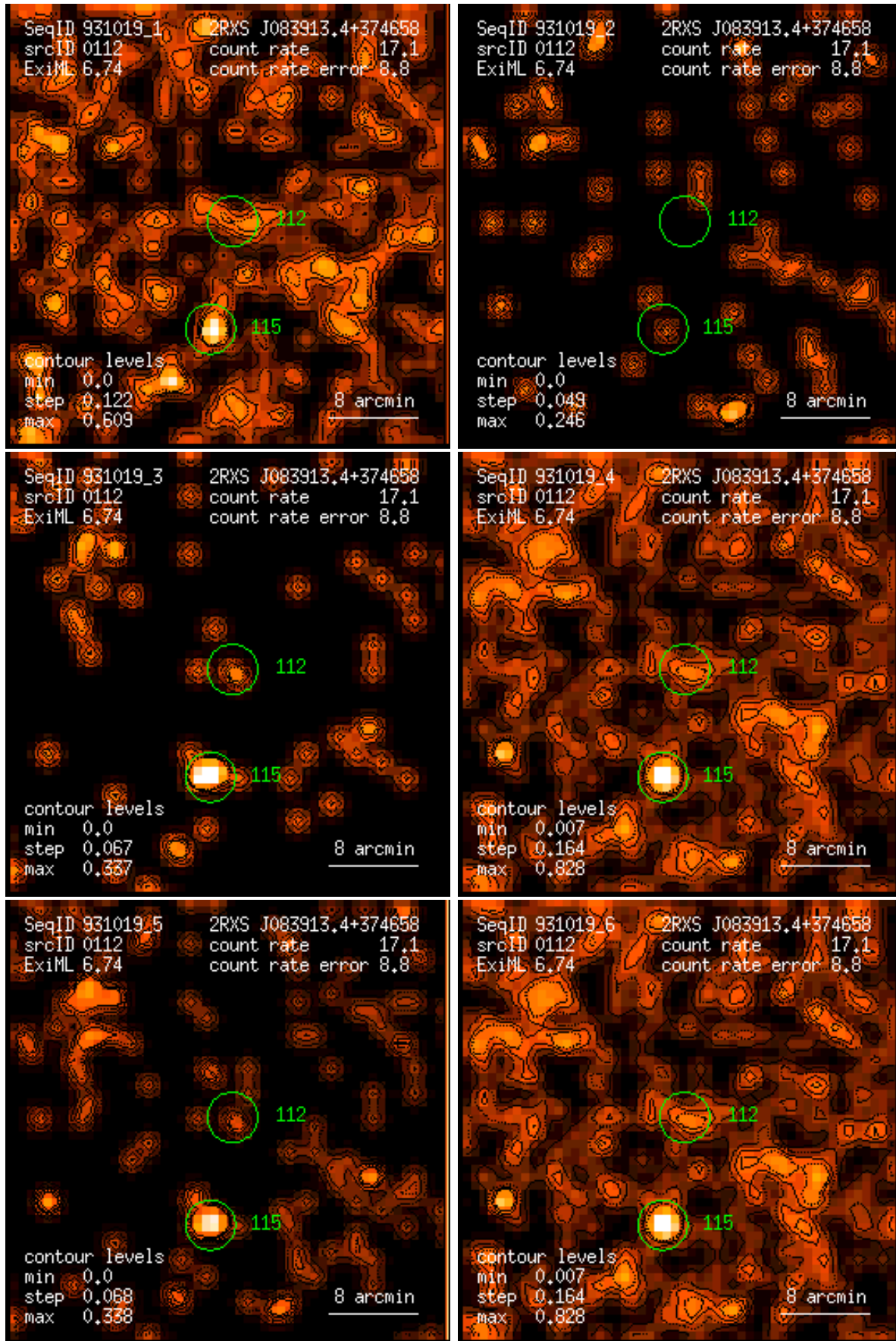
Figure 112: RASS 931019: detection 0112: band rate images, Gaussian filter: (1) PSPC channels 11 – 41, (2) 52 – 90, (3) 91 – 201, (4) 11 – 235, (5) 52 – 201, (6) 11 – 201. Broad band rates in counts/ks. Band rate contour levels in counts/ks/arcmin 2 .
