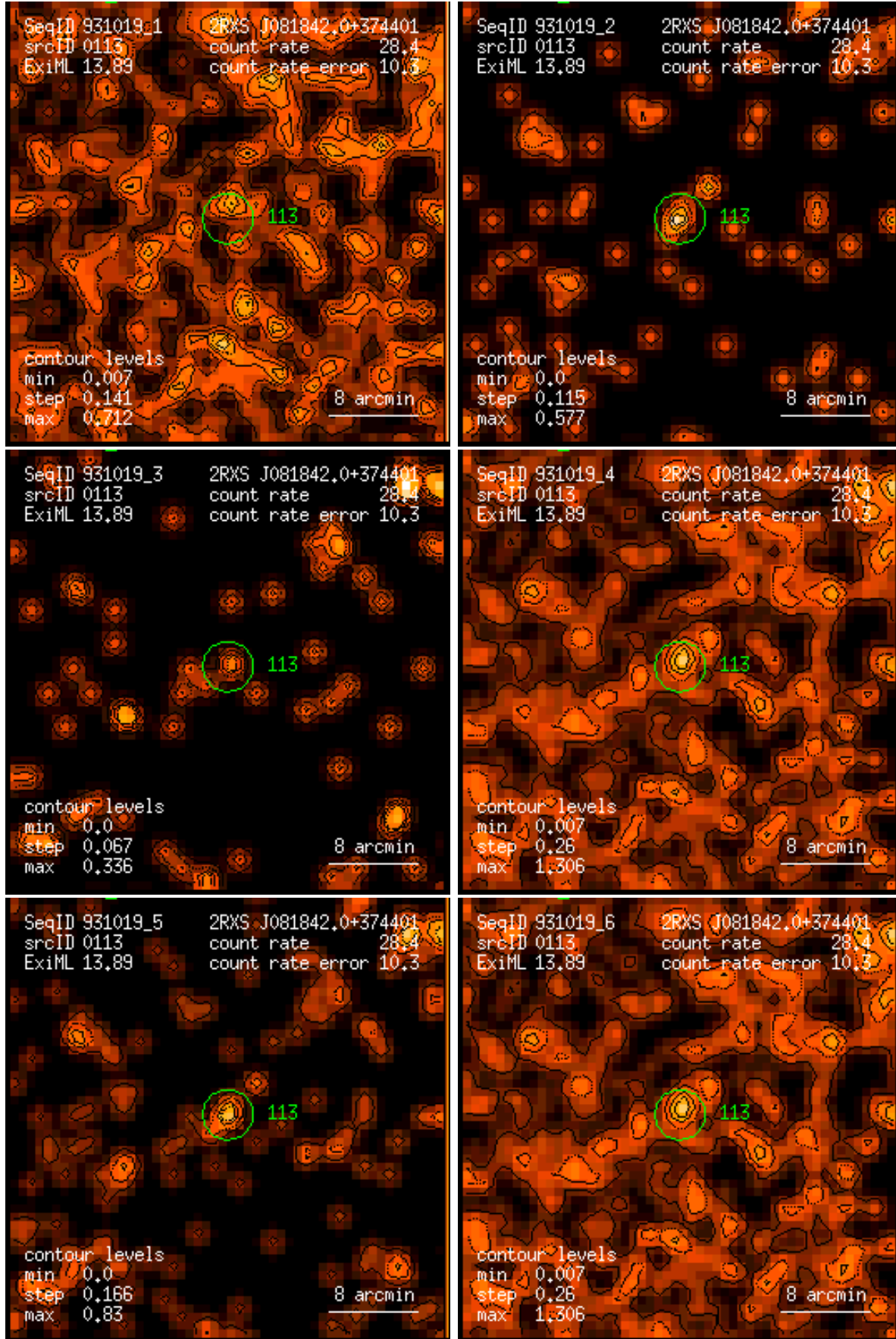
Figure 113: RASS 931019: detection 0113: band rate images, Gaussian filter: (1) PSPC channels 11 – 41, (2) 52 – 90, (3) 91 – 201, (4) 11 – 235, (5) 52 – 201, (6) 11 – 201. Broad band rates in counts/ks. Band rate contour levels in counts/ks/arcmin 2 .
