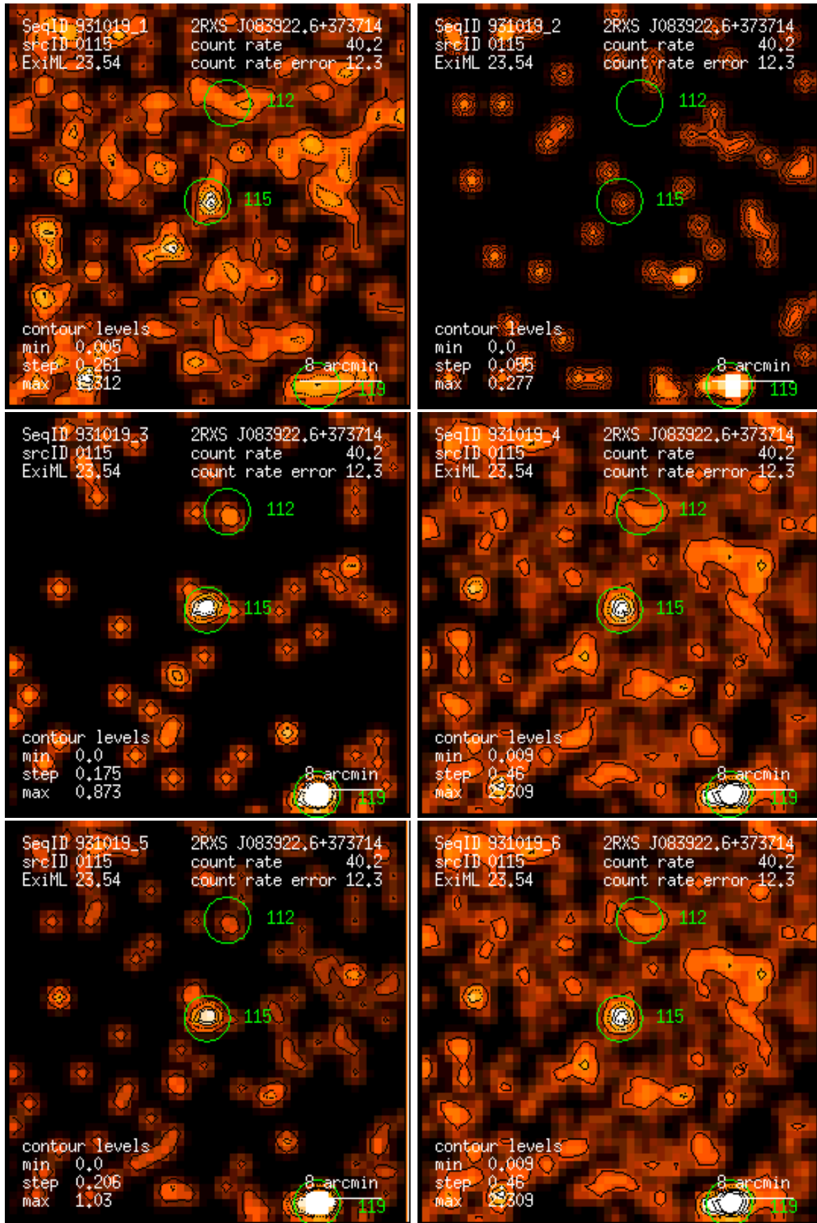
Figure 115: RASS 931019: detection 0115: band rate images, Gaussian filter: (1) PSPC channels 11 – 41, (2) 52 – 90, (3) 91 – 201, (4) 11 – 235, (5) 52 – 201, (6) 11 – 201. Broad band rates in counts/ks. Band rate contour levels in counts/ks/arcmin 2 .
