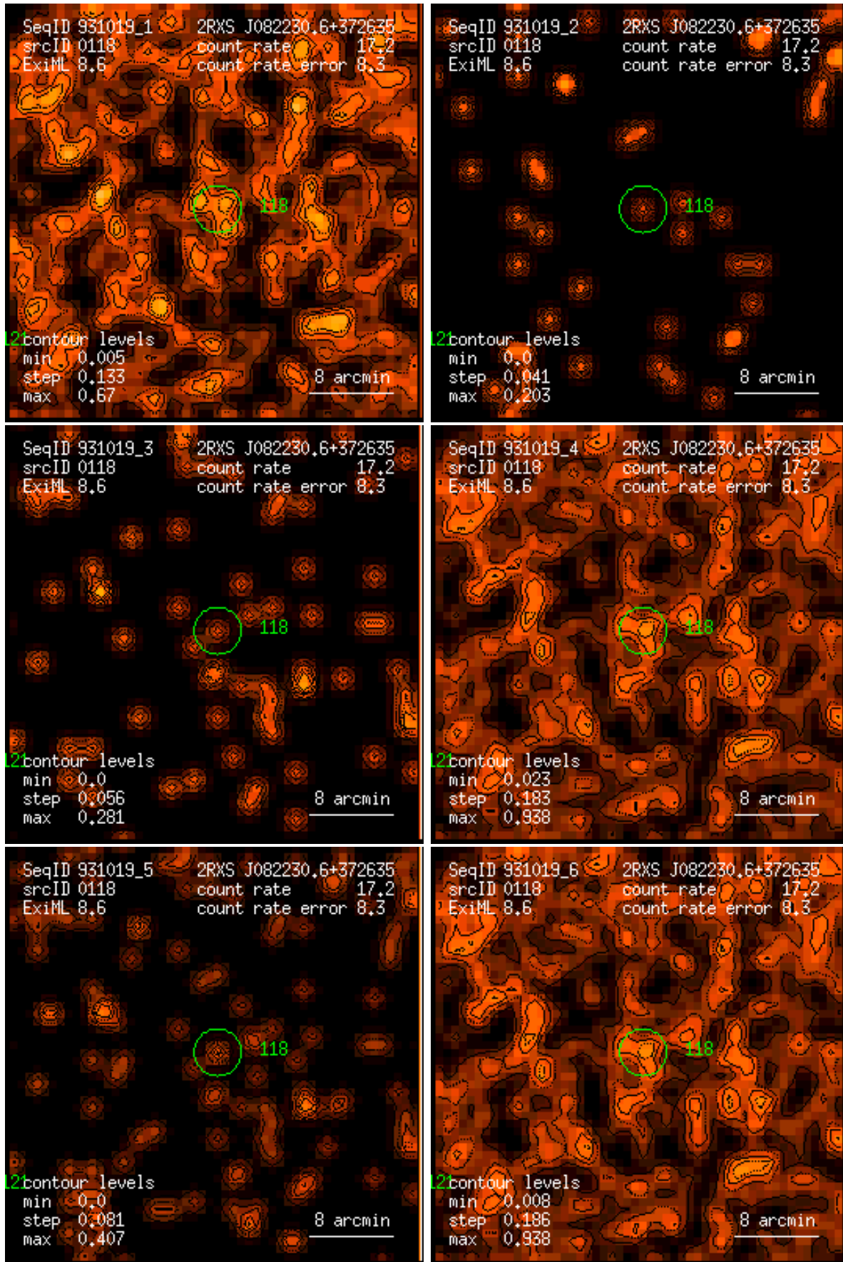
Figure 118: RASS 931019: detection 0118: band rate images, Gaussian filter: (1) PSPC channels 11 – 41, (2) 52 – 90, (3) 91 – 201, (4) 11 – 235, (5) 52 – 201, (6) 11 – 201. Broad band rates in counts/ks. Band rate contour levels in counts/ks/arcmin 2 .
