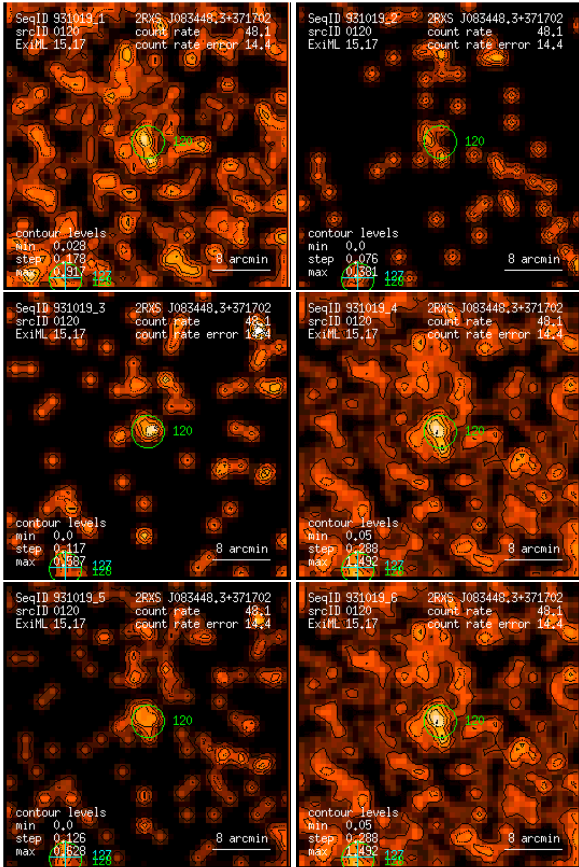
Figure 120: RASS 931019: detection 0120: band rate images, Gaussian filter: (1) PSPC channels 11 – 41, (2) 52 – 90, (3) 91 – 201, (4) 11 – 235, (5) 52 – 201, (6) 11 – 201. Broad band rates in counts/ks. Band rate contour levels in counts/ks/arcmin 2 .
