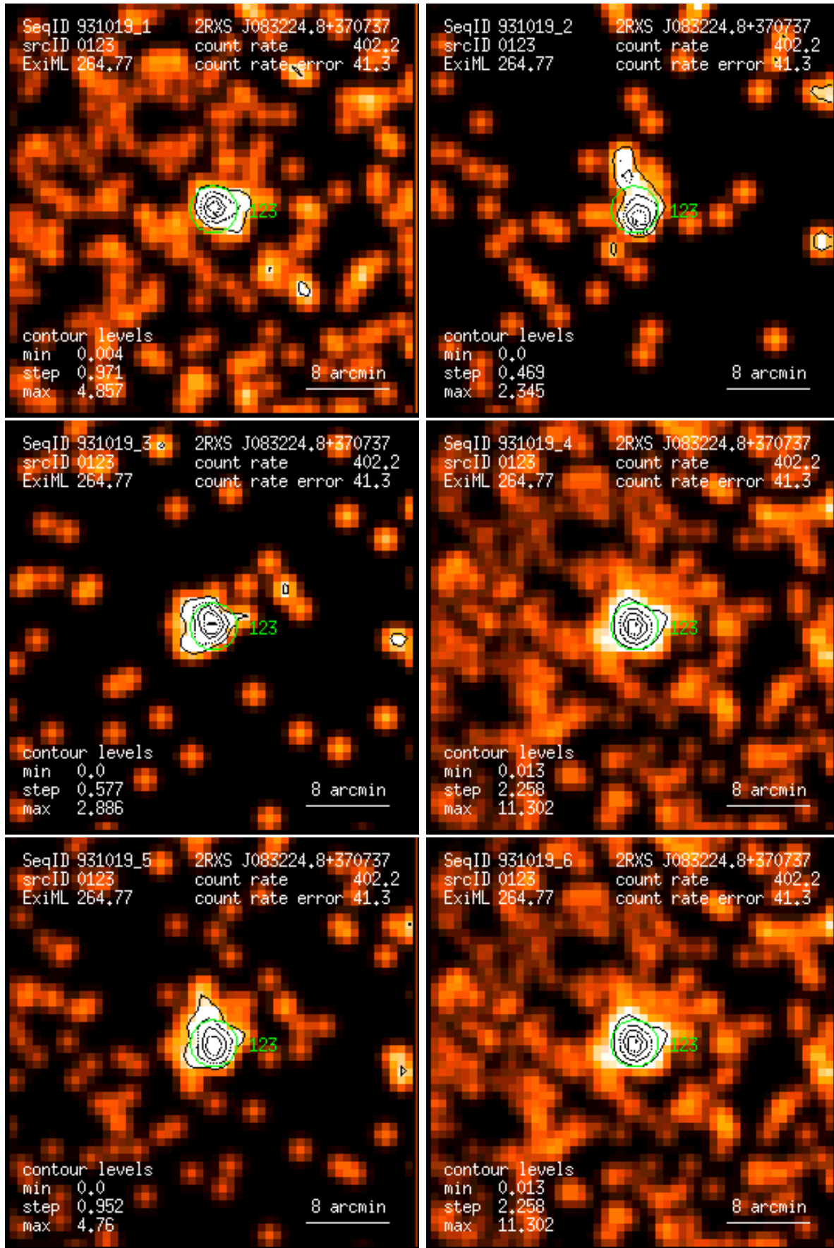
Figure 123: RASS 931019: detection 0123: band rate images, Gaussian filter: (1) PSPC channels 11 – 41, (2) 52 – 90, (3) 91 – 201, (4) 11 – 235, (5) 52 – 201, (6) 11 – 201. Broad band rates in counts/ks. Band rate contour levels in counts/ks/arcmin 2 .
