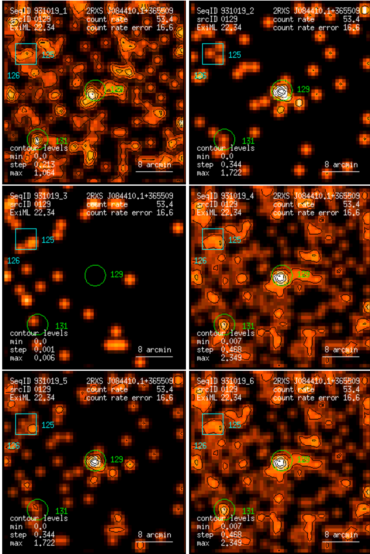
Figure 129: RASS 931019: detection 0129: band rate images, Gaussian filter: (1) PSPC channels 11 – 41, (2) 52 – 90, (3) 91 – 201, (4) 11 – 235, (5) 52 – 201, (6) 11 – 201. Broad band rates in counts/ks. Band rate contour levels in counts/ks/arcmin 2 .
