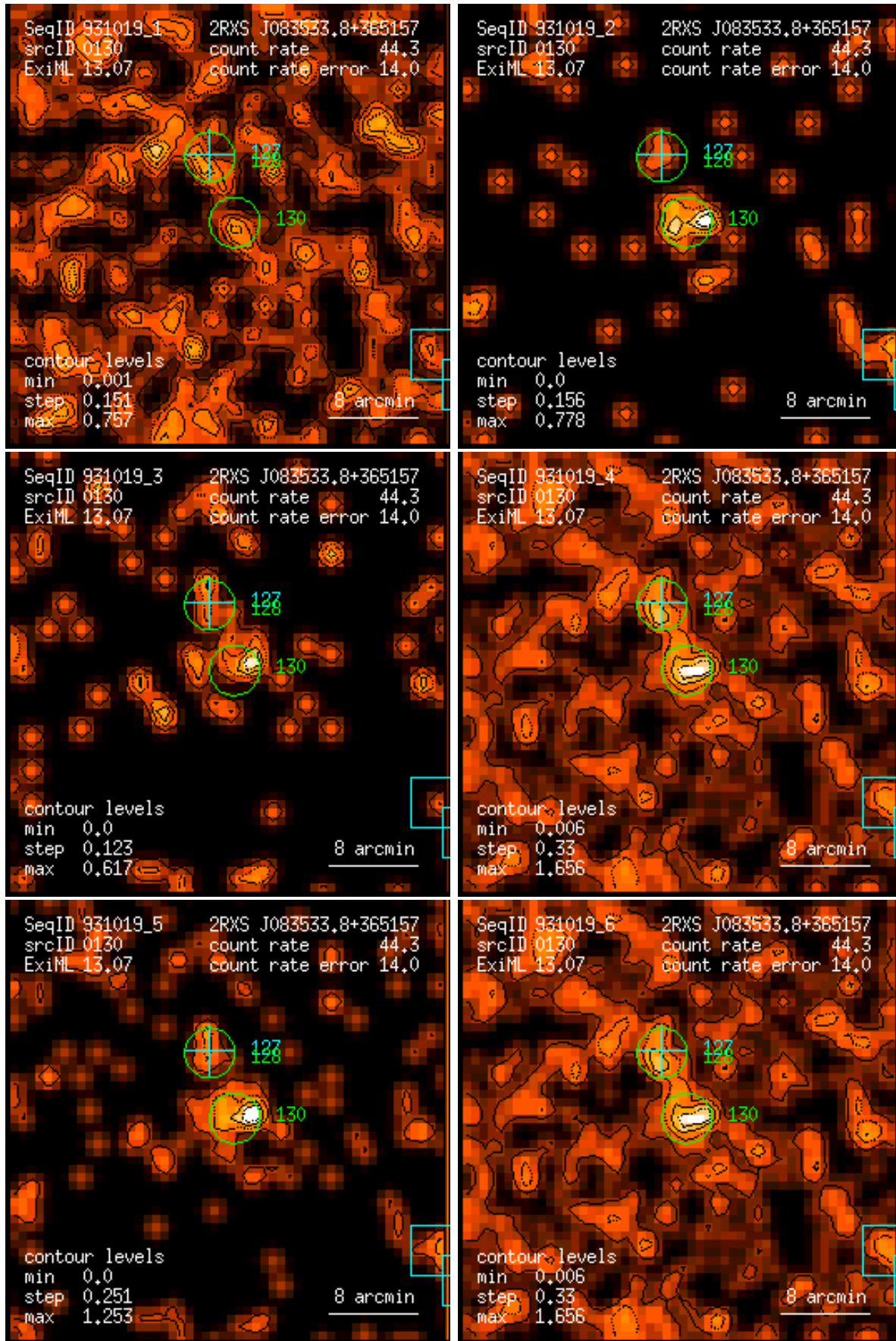
Figure 130: RASS 931019: detection 0130: band rate images, Gaussian filter: (1) PSPC channels 11 – 41, (2) 52 – 90, (3) 91 – 201, (4) 11 – 235, (5) 52 – 201, (6) 11 – 201. Broad band rates in counts/ks. Band rate contour levels in counts/ks/arcmin 2 .
