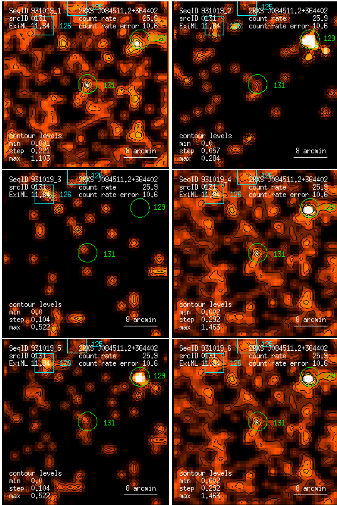
Figure 131: RASS 931019: detection 0131: band rate images, Gaussian filter: (1) PSPC channels 11 – 41, (2) 52 – 90, (3) 91 – 201, (4) 11 – 235, (5) 52 – 201, (6) 11 – 201. Broad band rates in counts/ks. Band rate contour levels in counts/ks/arcmin 2 .
