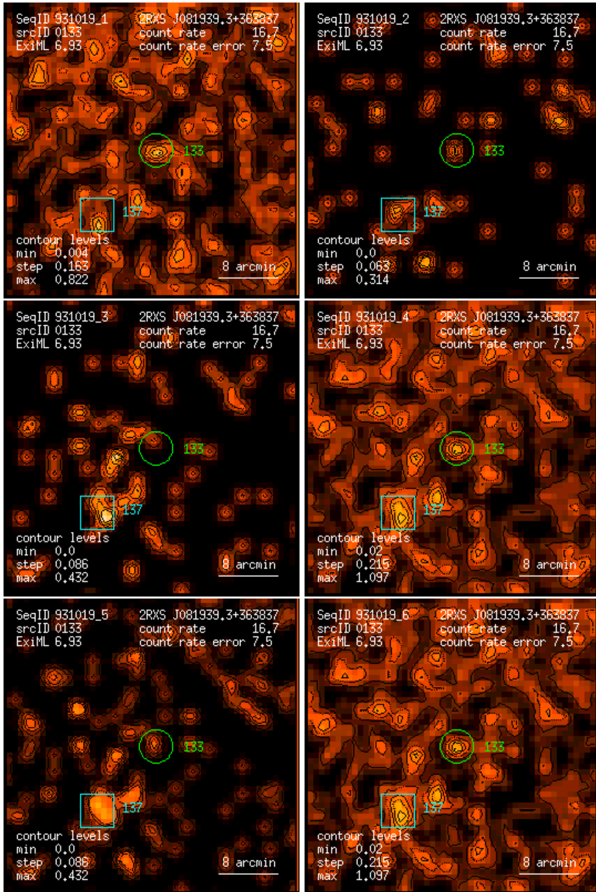
Figure 133: RASS 931019: detection 0133: band rate images, Gaussian filter: (1) PSPC channels 11 – 41, (2) 52 – 90, (3) 91 – 201, (4) 11 – 235, (5) 52 – 201, (6) 11 – 201. Broad band rates in counts/ks. Band rate contour levels in counts/ks/arcmin 2 .
