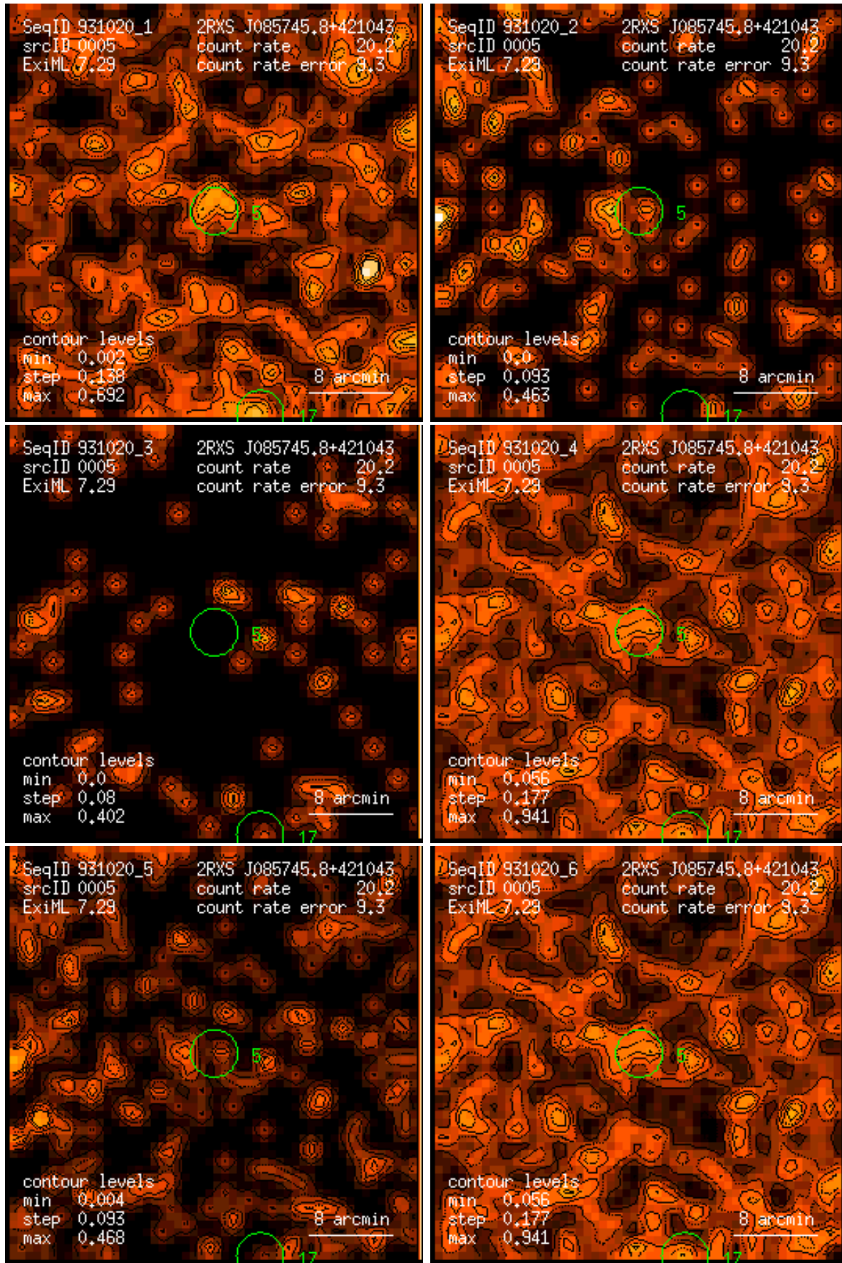
Figure 5: RASS 931020: detection 0005: band rate images, Gaussian filter: (1) PSPC channels 11 – 41, (2) 52 – 90, (3) 91 – 201, (4) 11 – 235, (5) 52 – 201, (6) 11 – 201. Broad band rates in counts/ks. Band rate contour levels in counts/ks/arcmin 2 .
