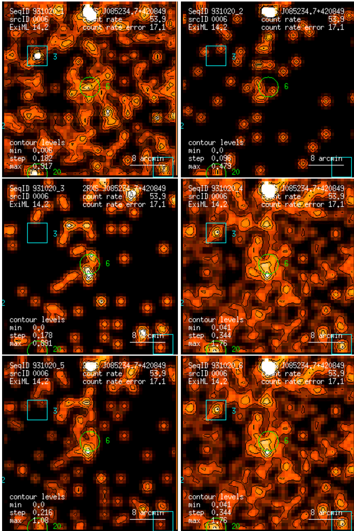
Figure 6: RASS 931020: detection 0006: band rate images, Gaussian filter: (1) PSPC channels 11 – 41, (2) 52 – 90, (3) 91 – 201, (4) 11 – 235, (5) 52 – 201, (6) 11 – 201. Broad band rates in counts/ks. Band rate contour levels in counts/ks/arcmin 2 .
