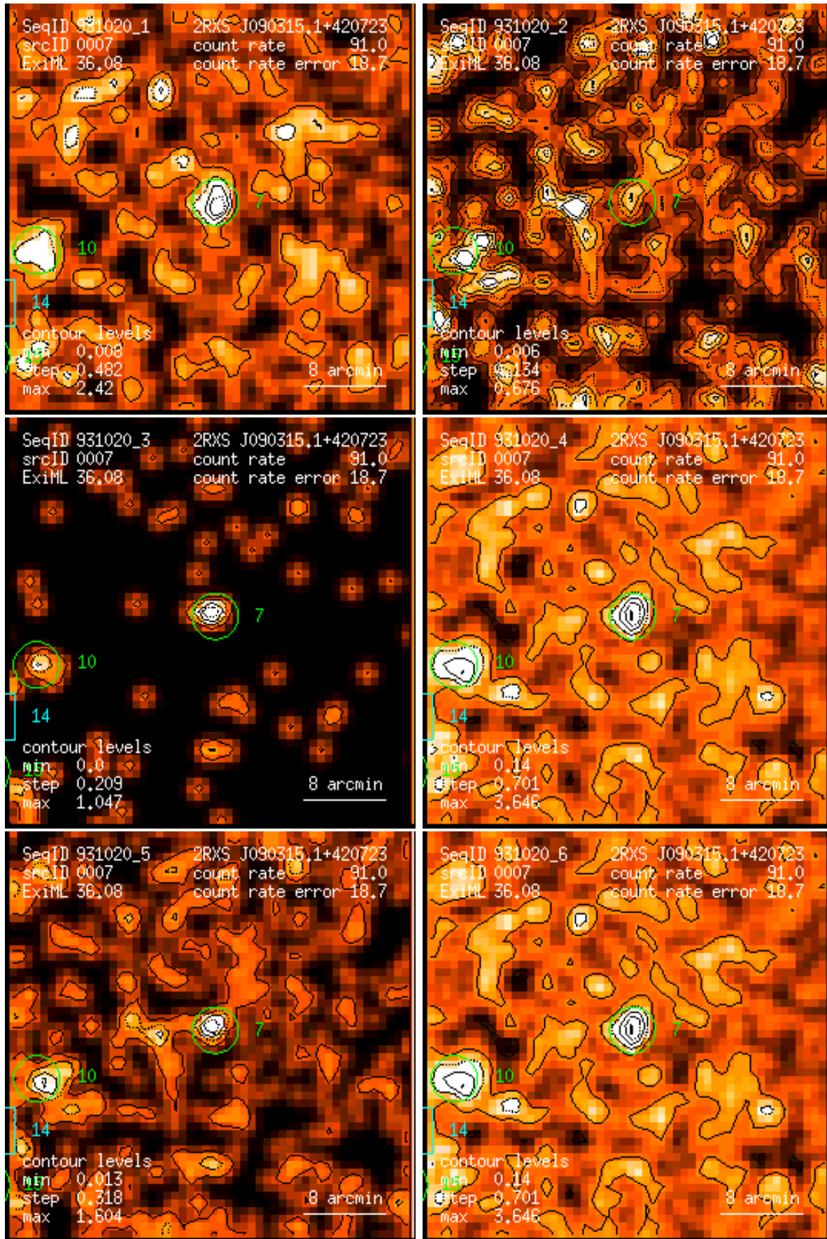
Figure 7: RASS 931020: detection 0007: band rate images, Gaussian filter: (1) PSPC channels 11 – 41, (2) 52 – 90, (3) 91 – 201, (4) 11 – 235, (5) 52 – 201, (6) 11 – 201. Broad band rates in counts/ks. Band rate contour levels in counts/ks/arcmin 2 .
