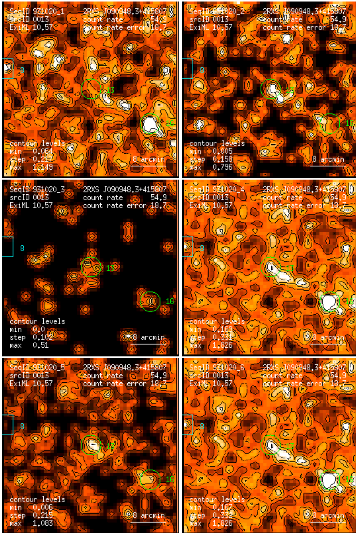
Figure 13: RASS 931020: detection 0013: band rate images, Gaussian filter: (1) PSPC channels 11 – 41, (2) 52 – 90, (3) 91 – 201, (4) 11 – 235, (5) 52 – 201, (6) 11 – 201. Broad band rates in counts/ks. Band rate contour levels in counts/ks/arcmin 2 .
