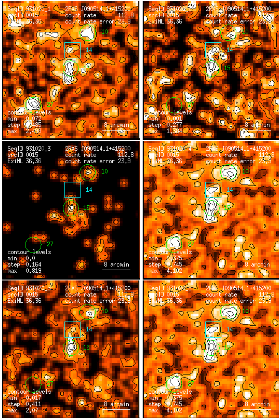
Figure 15: RASS 931020: detection 0015: band rate images, Gaussian filter: (1) PSPC channels 11 – 41, (2) 52 – 90, (3) 91 – 201, (4) 11 – 235, (5) 52 – 201, (6) 11 – 201. Broad band rates in counts/ks. Band rate contour levels in counts/ks/arcmin 2 .
