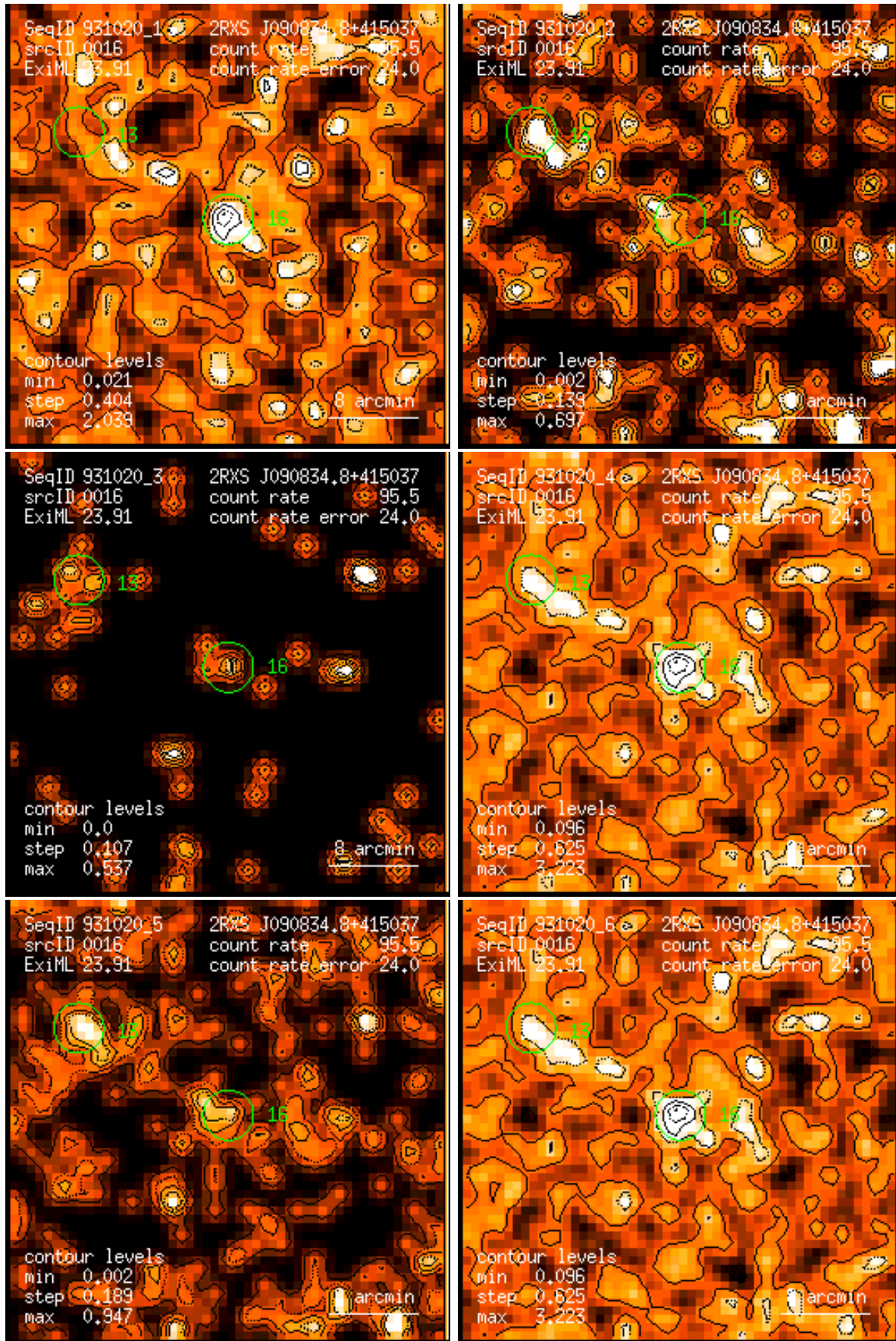
Figure 16: RASS 931020: detection 0016: band rate images, Gaussian filter: (1) PSPC channels 11 – 41, (2) 52 – 90, (3) 91 – 201, (4) 11 – 235, (5) 52 – 201, (6) 11 – 201. Broad band rates in counts/ks. Band rate contour levels in counts/ks/arcmin 2 .
