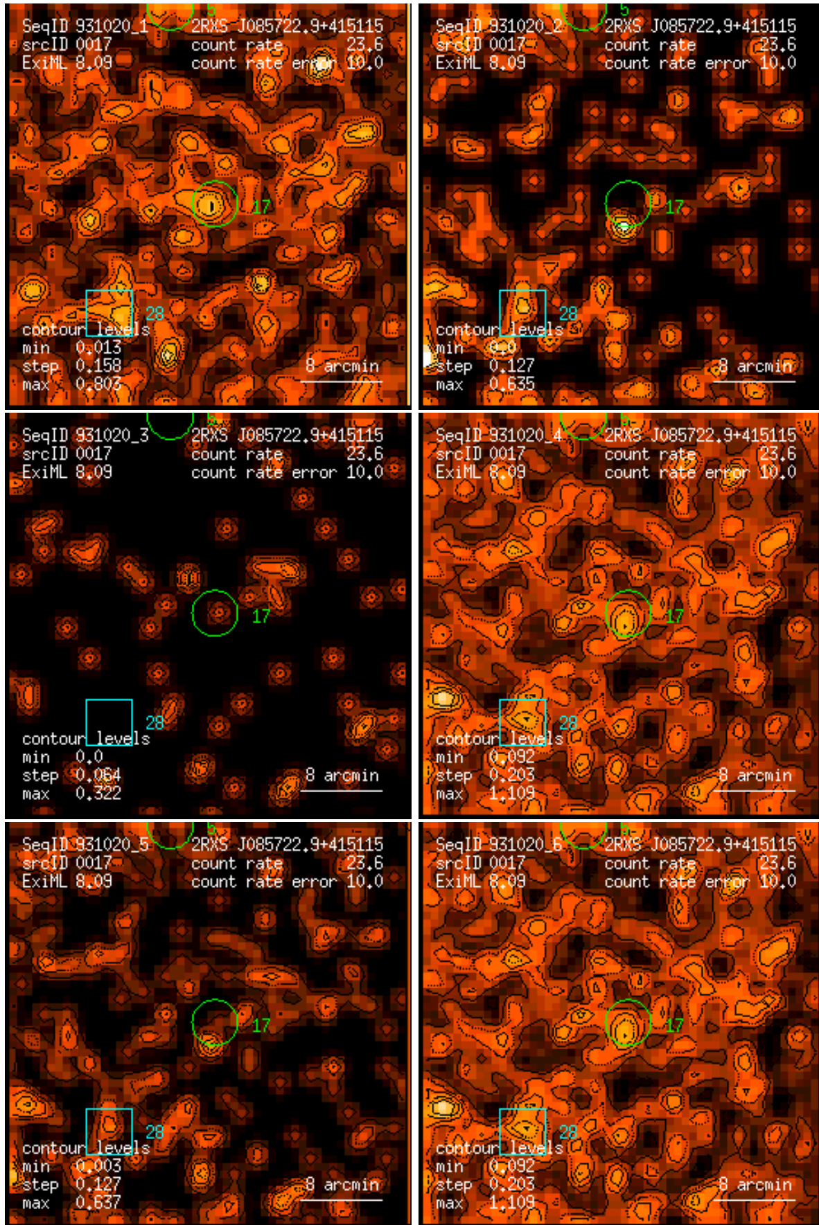
Figure 17: RASS 931020: detection 0017: band rate images, Gaussian filter: (1) PSPC channels 11 – 41, (2) 52 – 90, (3) 91 – 201, (4) 11 – 235, (5) 52 – 201, (6) 11 – 201. Broad band rates in counts/ks. Band rate contour levels in counts/ks/arcmin 2 .
