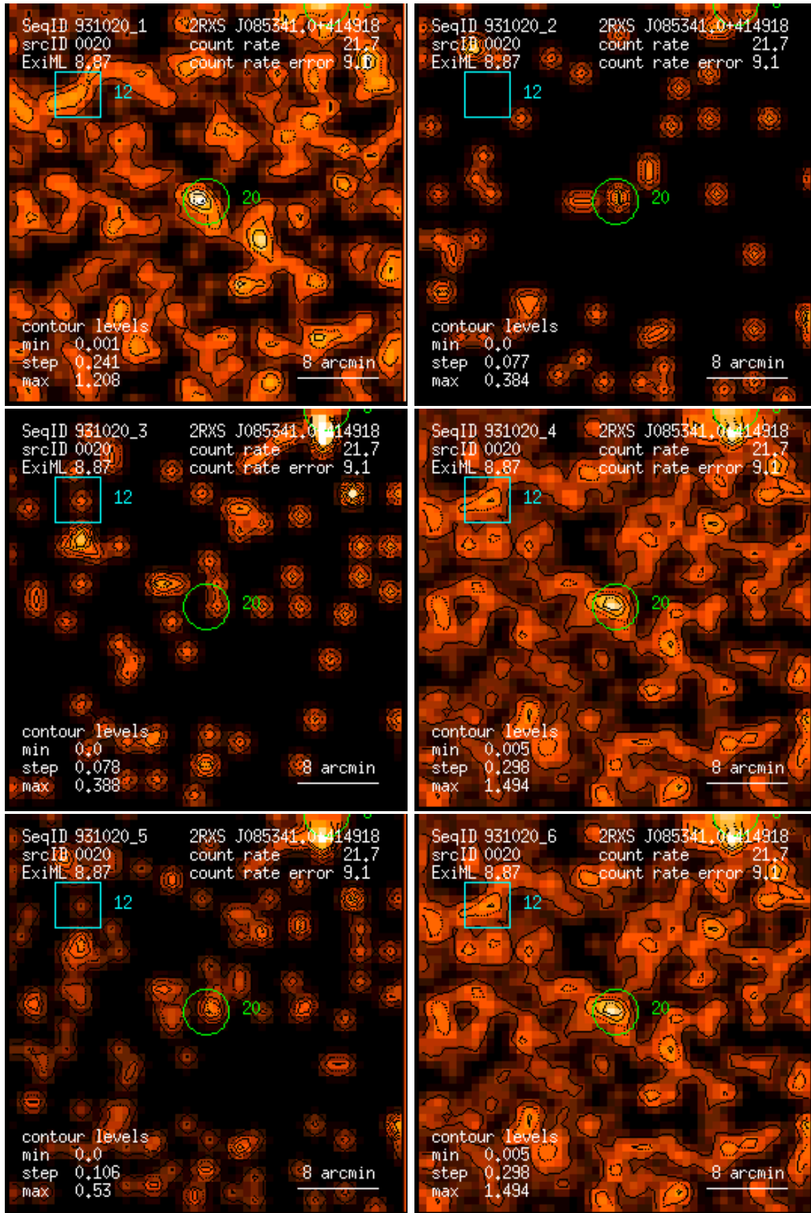
Figure 20: RASS 931020: detection 0020: band rate images, Gaussian filter: (1) PSPC channels 11 – 41, (2) 52 – 90, (3) 91 – 201, (4) 11 – 235, (5) 52 – 201, (6) 11 – 201. Broad band rates in counts/ks. Band rate contour levels in counts/ks/arcmin 2 .
