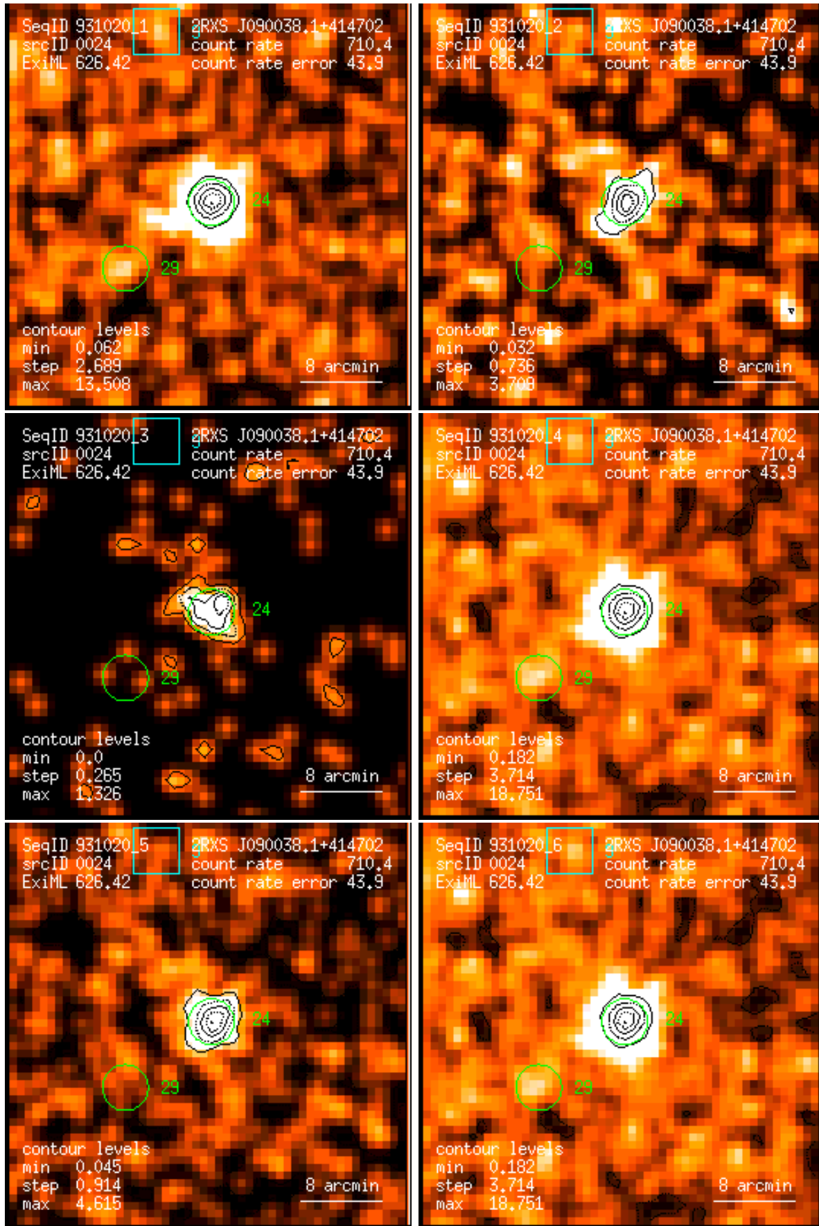
Figure 24: RASS 931020: detection 0024: band rate images, Gaussian filter: (1) PSPC channels 11 – 41, (2) 52 – 90, (3) 91 – 201, (4) 11 – 235, (5) 52 – 201, (6) 11 – 201. Broad band rates in counts/ks. Band rate contour levels in counts/ks/arcmin 2 .
