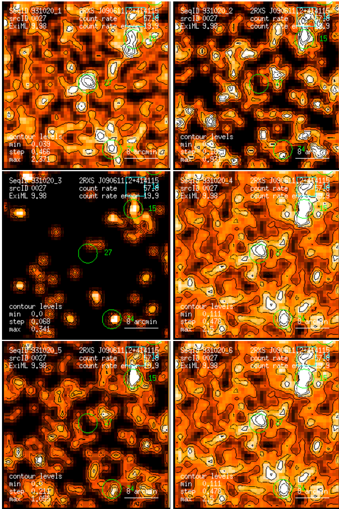
Figure 27: RASS 931020: detection 0027: band rate images, Gaussian filter: (1) PSPC channels 11 – 41, (2) 52 – 90, (3) 91 – 201, (4) 11 – 235, (5) 52 – 201, (6) 11 – 201. Broad band rates in counts/ks. Band rate contour levels in counts/ks/arcmin 2 .
