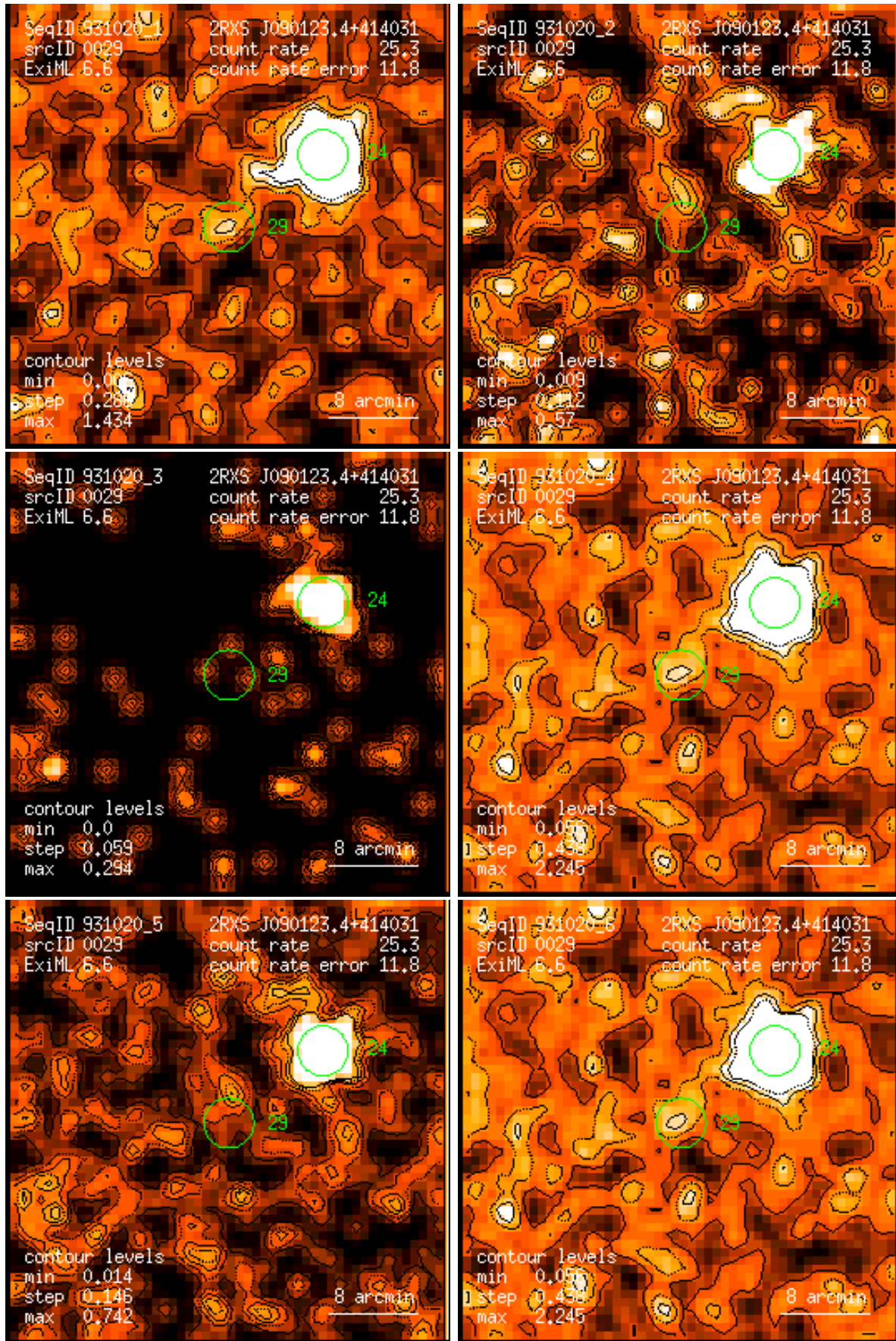
Figure 29: RASS 931020: detection 0029: band rate images, Gaussian filter: (1) PSPC channels 11 – 41, (2) 52 – 90, (3) 91 – 201, (4) 11 – 235, (5) 52 – 201, (6) 11 – 201. Broad band rates in counts/ks. Band rate contour levels in counts/ks/arcmin 2 .
