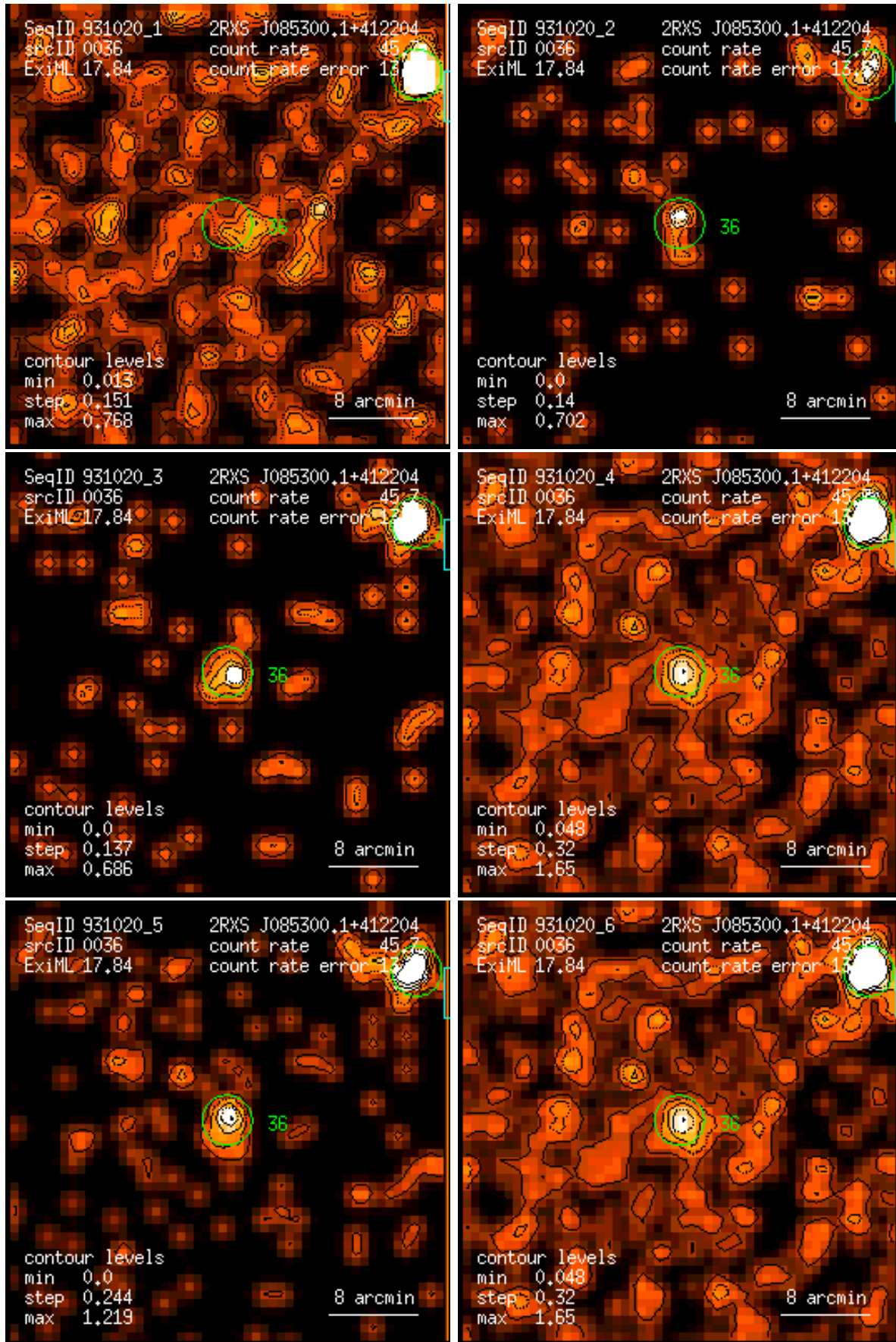
Figure 36: RASS 931020: detection 0036: band rate images, Gaussian filter: (1) PSPC channels 11 – 41, (2) 52 – 90, (3) 91 – 201, (4) 11 – 235, (5) 52 – 201, (6) 11 – 201. Broad band rates in counts/ks. Band rate contour levels in counts/ks/arcmin 2 .
