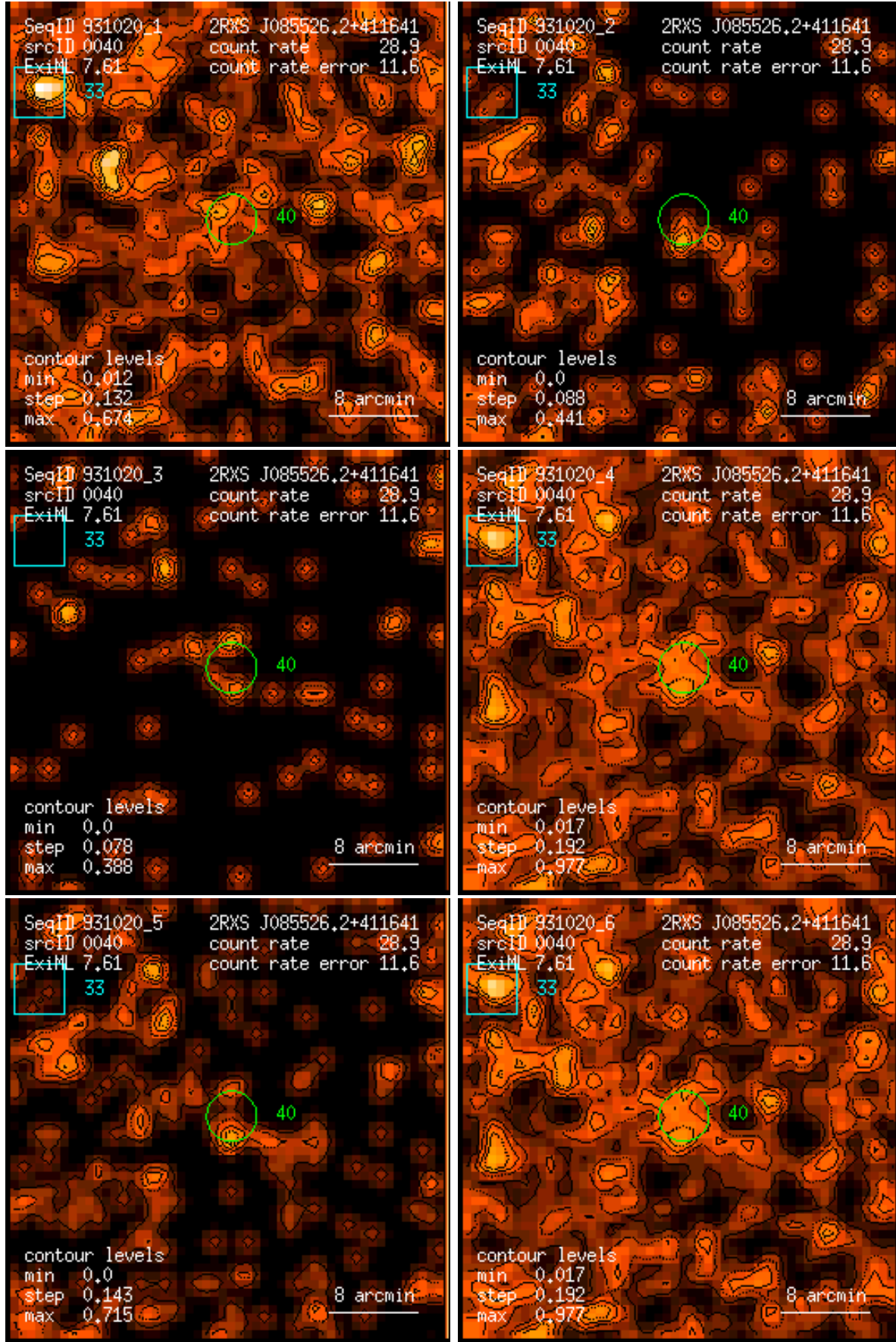
Figure 40: RASS 931020: detection 0040: band rate images, Gaussian filter: (1) PSPC channels 11 – 41, (2) 52 – 90, (3) 91 – 201, (4) 11 – 235, (5) 52 – 201, (6) 11 – 201. Broad band rates in counts/ks. Band rate contour levels in counts/ks/arcmin 2 .
