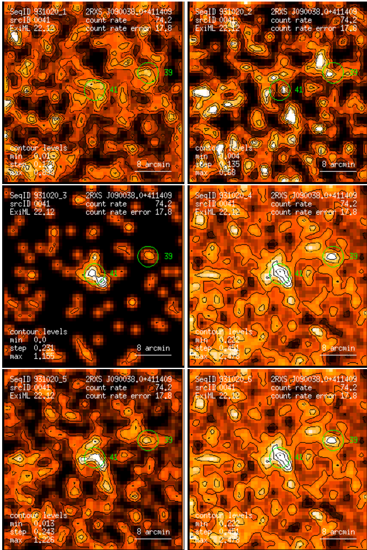
Figure 41: RASS 931020: detection 0041: band rate images, Gaussian filter: (1) PSPC channels 11 – 41, (2) 52 – 90, (3) 91 – 201, (4) 11 – 235, (5) 52 – 201, (6) 11 – 201. Broad band rates in counts/ks. Band rate contour levels in counts/ks/arcmin 2 .
