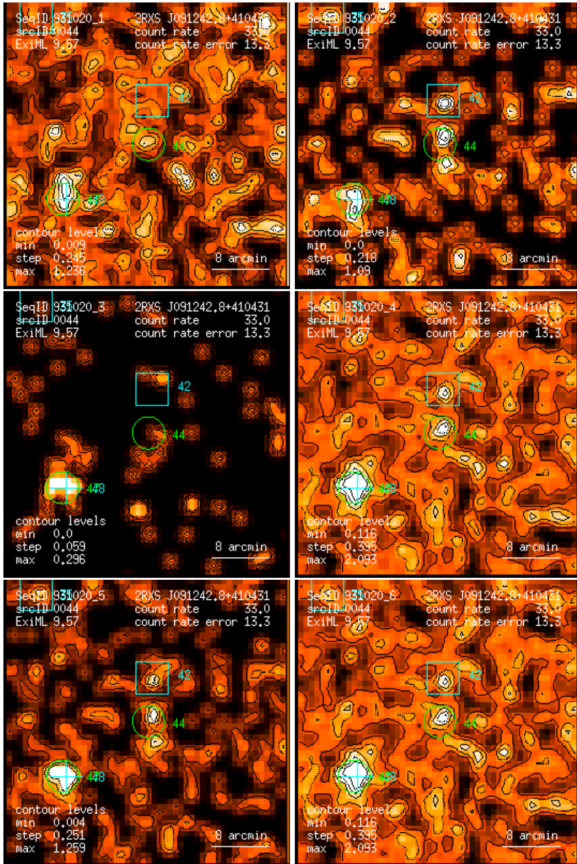
Figure 44: RASS 931020: detection 0044: band rate images, Gaussian filter: (1) PSPC channels 11 – 41, (2) 52 – 90, (3) 91 – 201, (4) 11 – 235, (5) 52 – 201, (6) 11 – 201. Broad band rates in counts/ks. Band rate contour levels in counts/ks/arcmin 2 .
