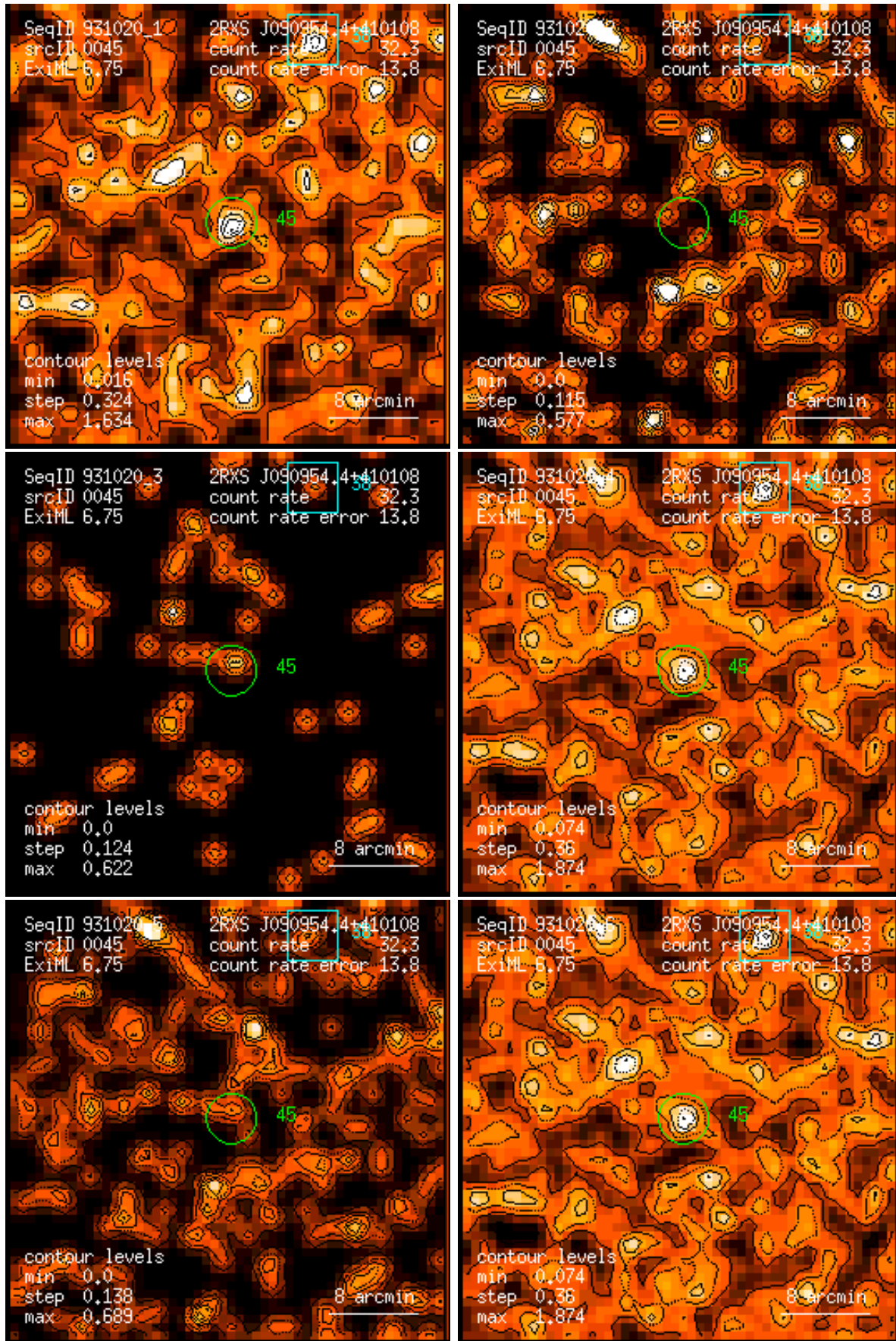
Figure 45: RASS 931020: detection 0045: band rate images, Gaussian filter: (1) PSPC channels 11 – 41, (2) 52 – 90, (3) 91 – 201, (4) 11 – 235, (5) 52 – 201, (6) 11 – 201. Broad band rates in counts/ks. Band rate contour levels in counts/ks/arcmin 2 .
