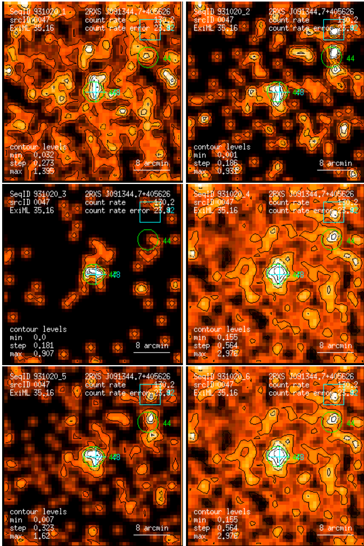
Figure 47: RASS 931020: detection 0047: band rate images, Gaussian filter: (1) PSPC channels 11 – 41, (2) 52 – 90, (3) 91 – 201, (4) 11 – 235, (5) 52 – 201, (6) 11 – 201. Broad band rates in counts/ks. Band rate contour levels in counts/ks/arcmin 2 .
