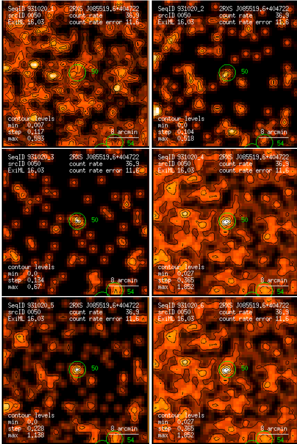
Figure 50: RASS 931020: detection 0050: band rate images, Gaussian filter: (1) PSPC channels 11 – 41, (2) 52 – 90, (3) 91 – 201, (4) 11 – 235, (5) 52 – 201, (6) 11 – 201. Broad band rates in counts/ks. Band rate contour levels in counts/ks/arcmin 2 .
