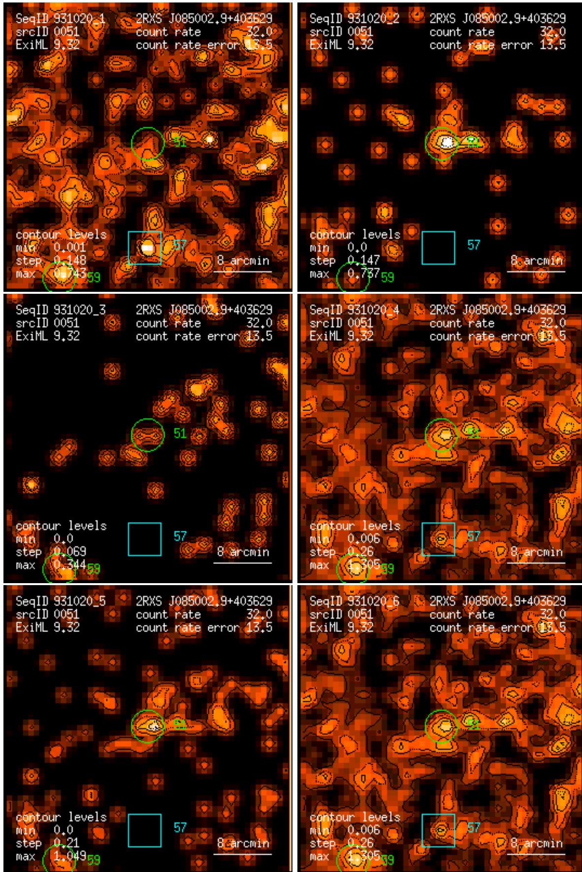
Figure 51: RASS 931020: detection 0051: band rate images, Gaussian filter: (1) PSPC channels 11 – 41, (2) 52 – 90, (3) 91 – 201, (4) 11 – 235, (5) 52 – 201, (6) 11 – 201. Broad band rates in counts/ks. Band rate contour levels in counts/ks/arcmin 2 .
