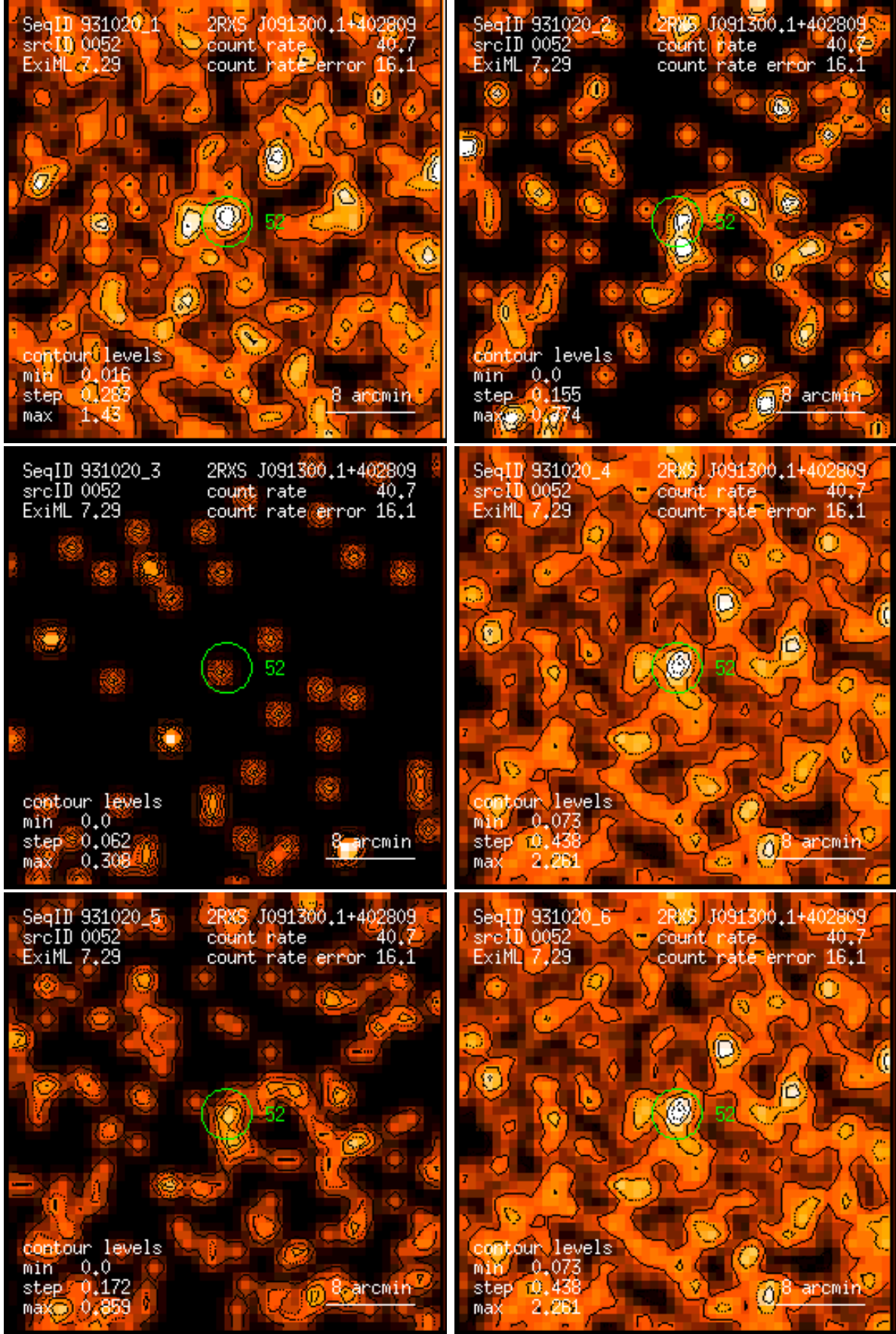
Figure 52: RASS 931020: detection 0052: band rate images, Gaussian filter: (1) PSPC channels 11 – 41, (2) 52 – 90, (3) 91 – 201, (4) 11 – 235, (5) 52 – 201, (6) 11 – 201. Broad band rates in counts/ks. Band rate contour levels in counts/ks/arcmin 2 .
