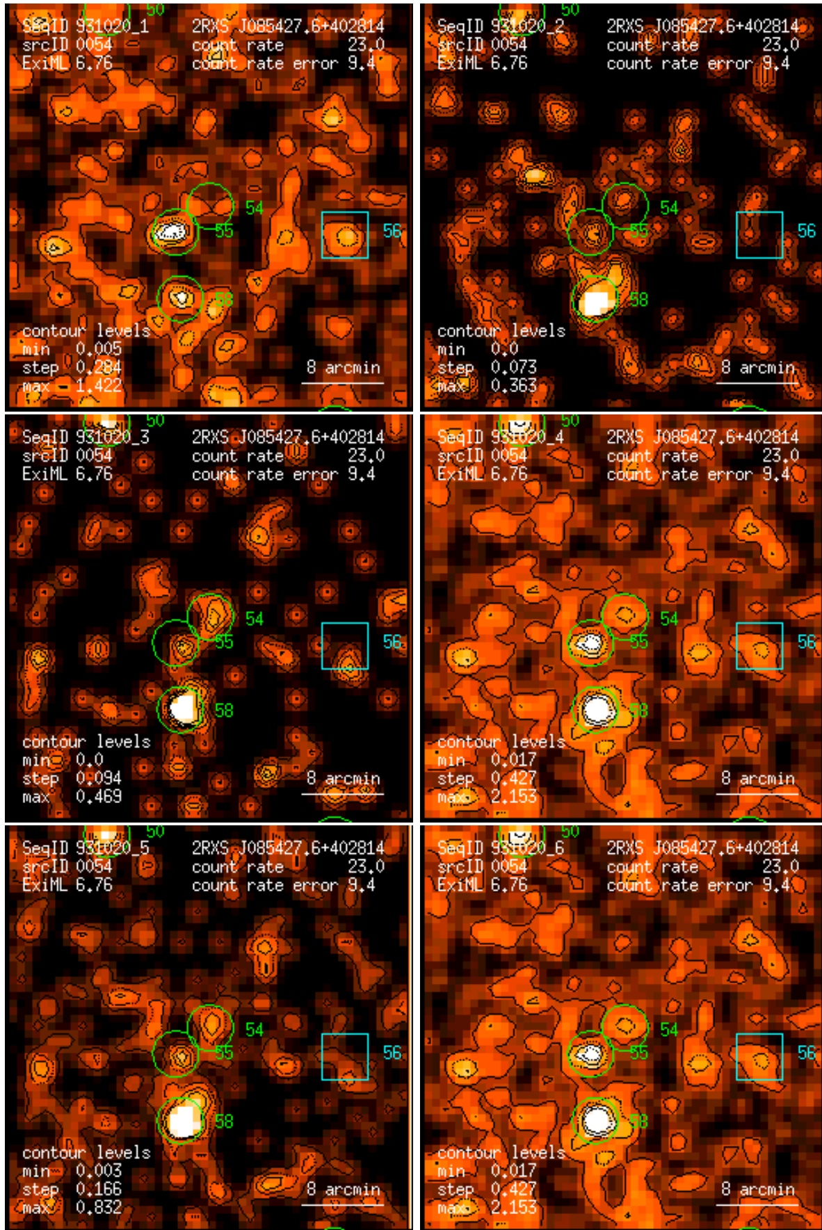
Figure 54: RASS 931020: detection 0054: band rate images, Gaussian filter: (1) PSPC channels 11 – 41, (2) 52 – 90, (3) 91 – 201, (4) 11 – 235, (5) 52 – 201, (6) 11 – 201. Broad band rates in counts/ks. Band rate contour levels in counts/ks/arcmin 2 .
