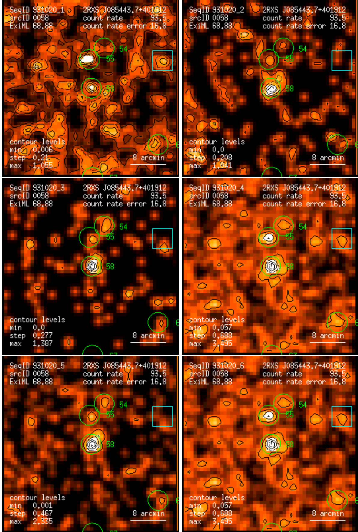
Figure 58: RASS 931020: detection 0058: band rate images, Gaussian filter: (1) PSPC channels 11 – 41, (2) 52 – 90, (3) 91 – 201, (4) 11 – 235, (5) 52 – 201, (6) 11 – 201. Broad band rates in counts/ks. Band rate contour levels in counts/ks/arcmin 2 .
