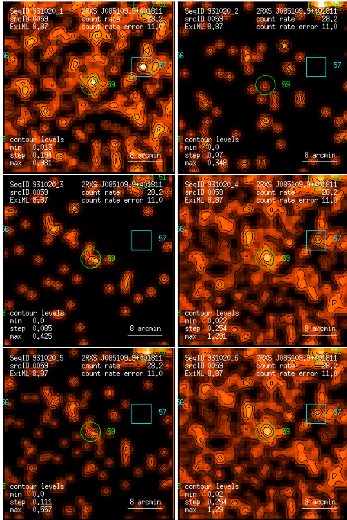
Figure 59: RASS 931020: detection 0059: band rate images, Gaussian filter: (1) PSPC channels 11 – 41, (2) 52 – 90, (3) 91 – 201, (4) 11 – 235, (5) 52 – 201, (6) 11 – 201. Broad band rates in counts/ks. Band rate contour levels in counts/ks/arcmin 2 .
