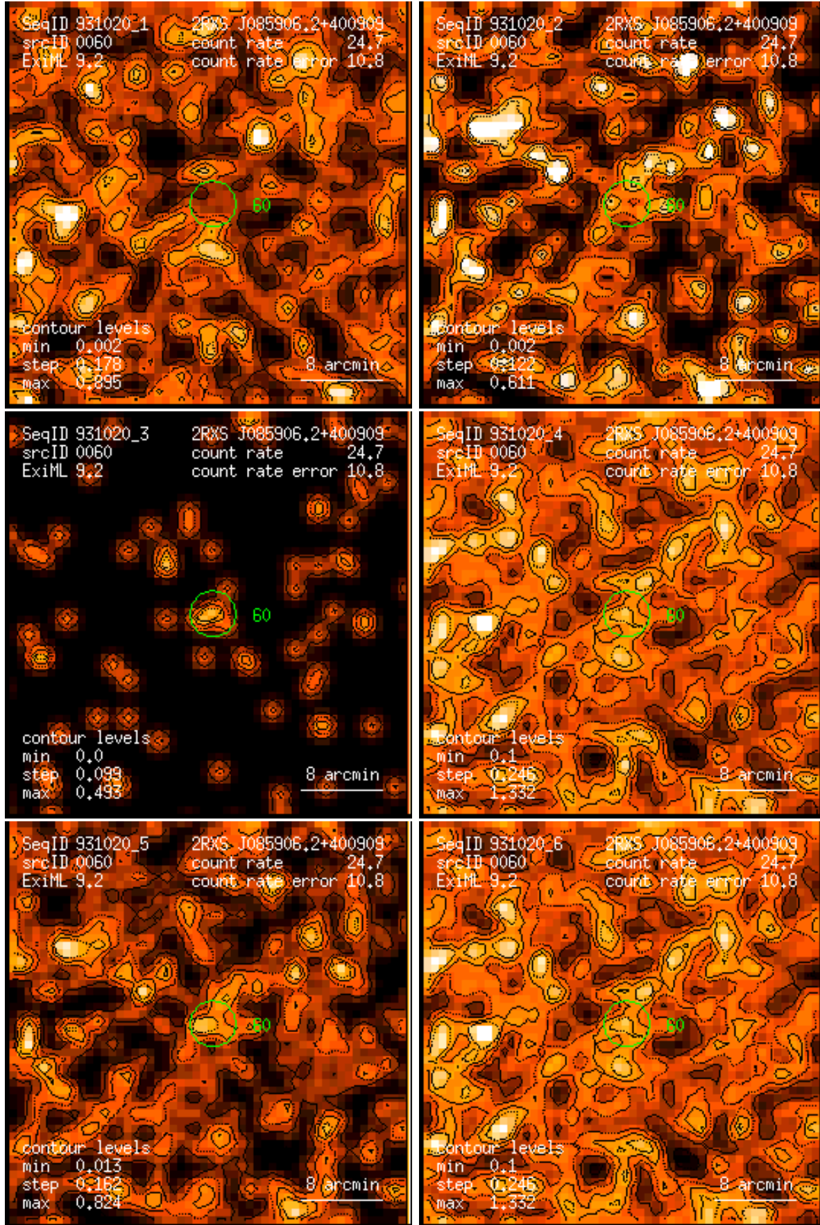
Figure 60: RASS 931020: detection 0060: band rate images, Gaussian filter: (1) PSPC channels 11 – 41, (2) 52 – 90, (3) 91 – 201, (4) 11 – 235, (5) 52 – 201, (6) 11 – 201. Broad band rates in counts/ks. Band rate contour levels in counts/ks/arcmin 2 .
