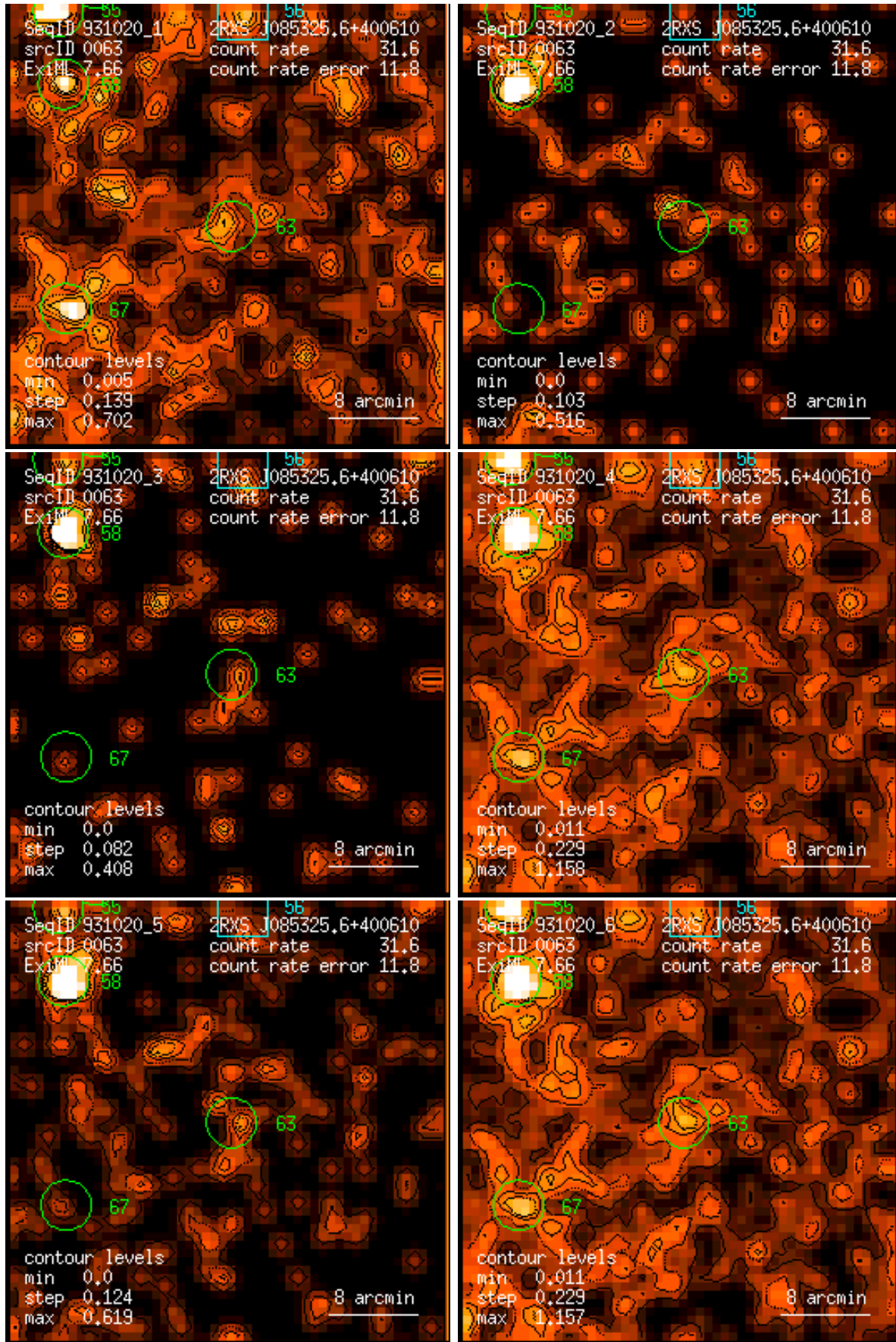
Figure 63: RASS 931020: detection 0063: band rate images, Gaussian filter: (1) PSPC channels 11 – 41, (2) 52 – 90, (3) 91 – 201, (4) 11 – 235, (5) 52 – 201, (6) 11 – 201. Broad band rates in counts/ks. Band rate contour levels in counts/ks/arcmin 2 .
