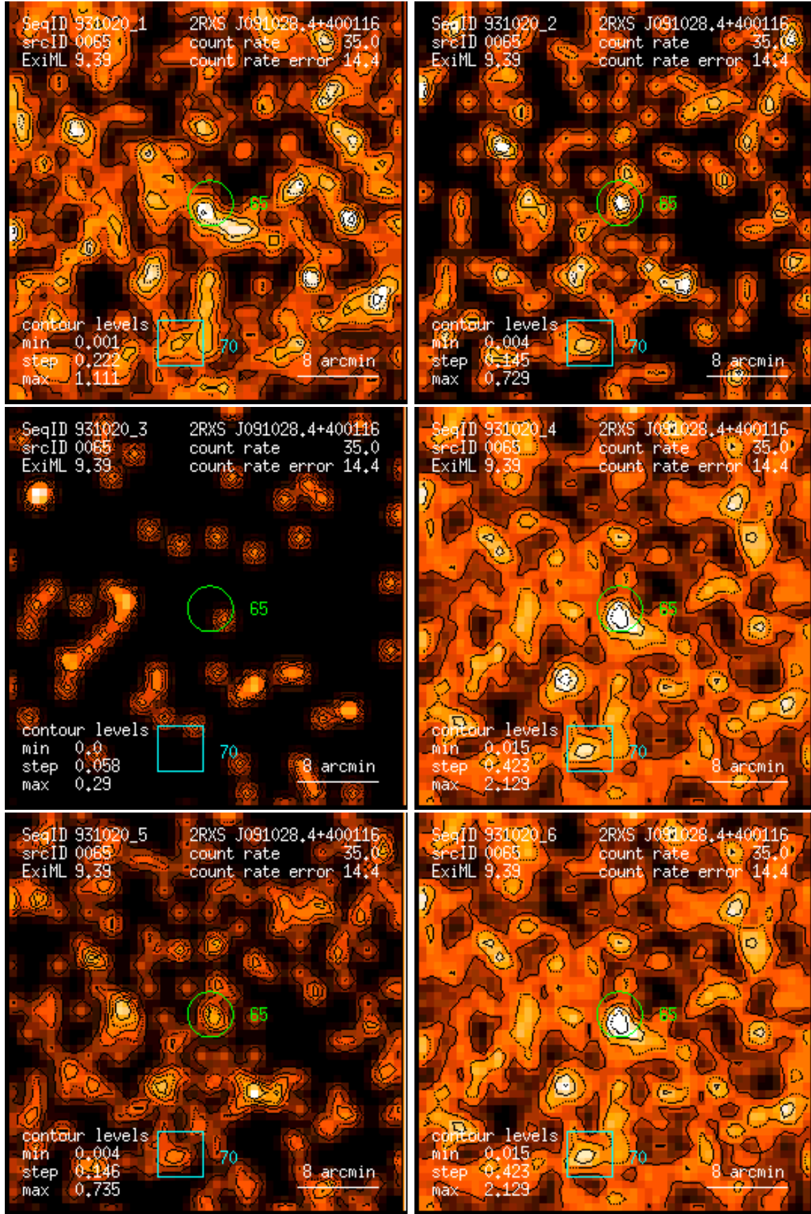
Figure 65: RASS 931020: detection 0065: band rate images, Gaussian filter: (1) PSPC channels 11 – 41, (2) 52 – 90, (3) 91 – 201, (4) 11 – 235, (5) 52 – 201, (6) 11 – 201. Broad band rates in counts/ks. Band rate contour levels in counts/ks/arcmin 2 .
