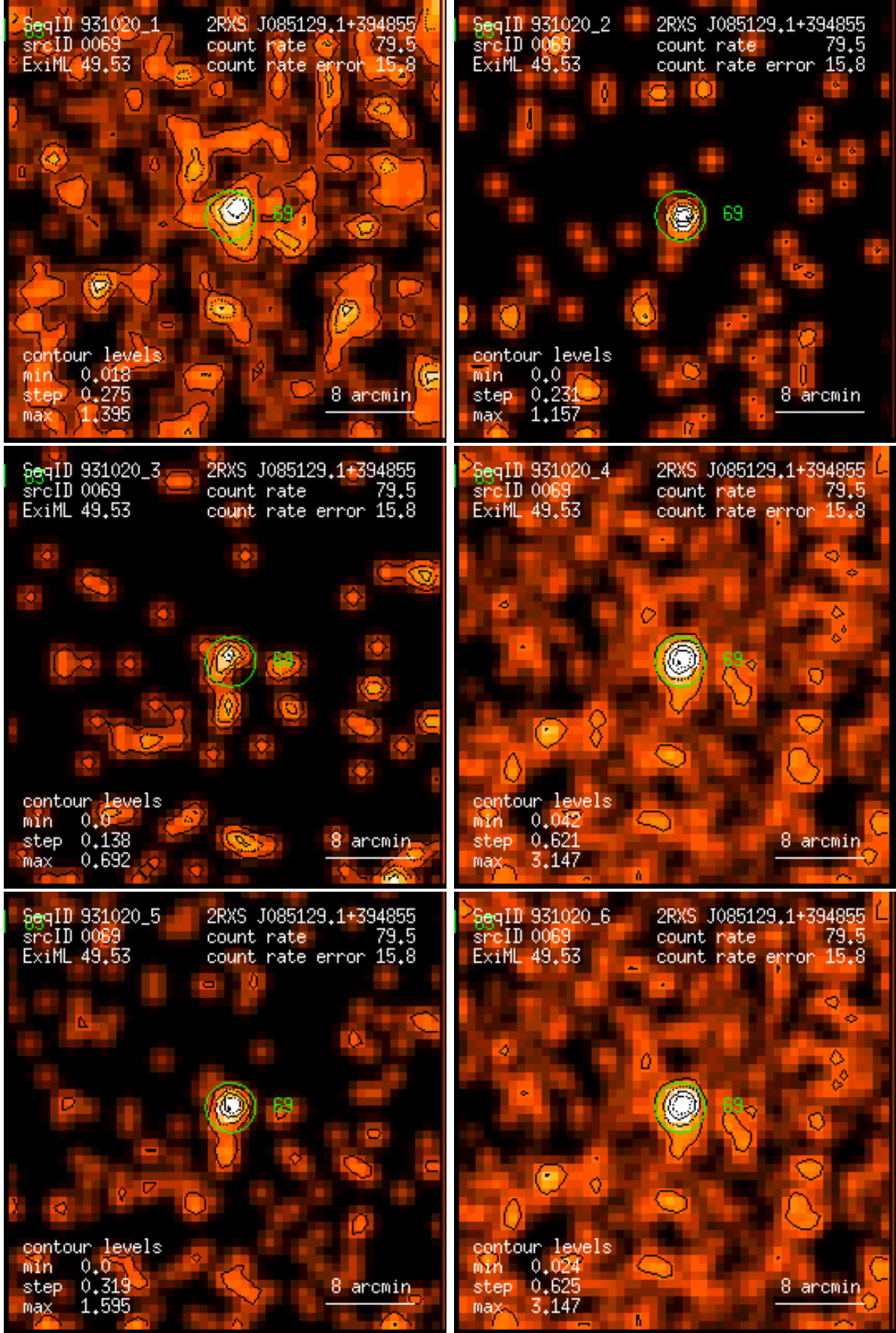
Figure 69: RASS 931020: detection 0069: band rate images, Gaussian filter: (1) PSPC channels 11 – 41, (2) 52 – 90, (3) 91 – 201, (4) 11 – 235, (5) 52 – 201, (6) 11 – 201. Broad band rates in counts/ks. Band rate contour levels in counts/ks/arcmin 2 .
