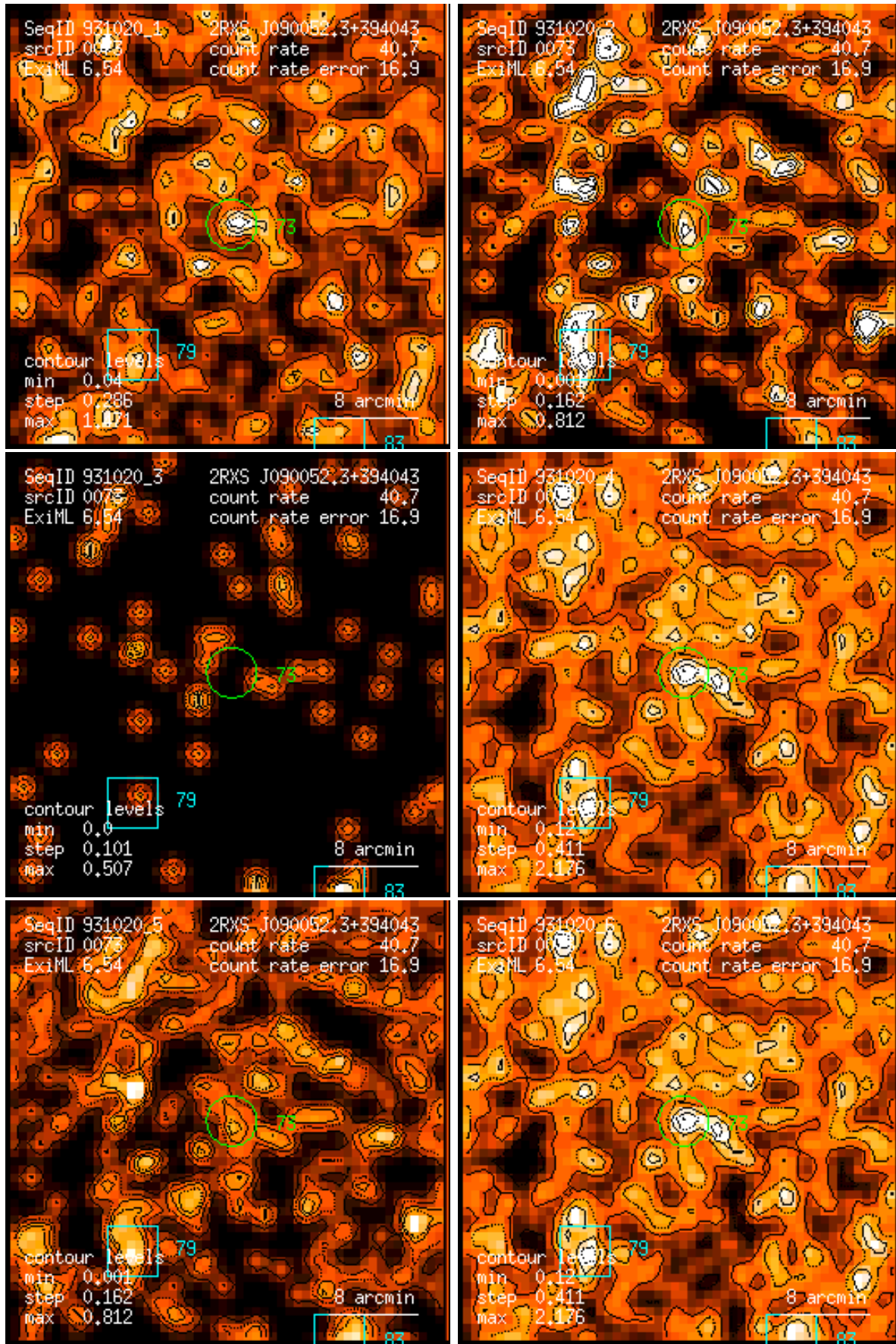
Figure 73: RASS 931020: detection 0073: band rate images, Gaussian filter: (1) PSPC channels 11 – 41, (2) 52 – 90, (3) 91 – 201, (4) 11 – 235, (5) 52 – 201, (6) 11 – 201. Broad band rates in counts/ks. Band rate contour levels in counts/ks/arcmin 2 .
