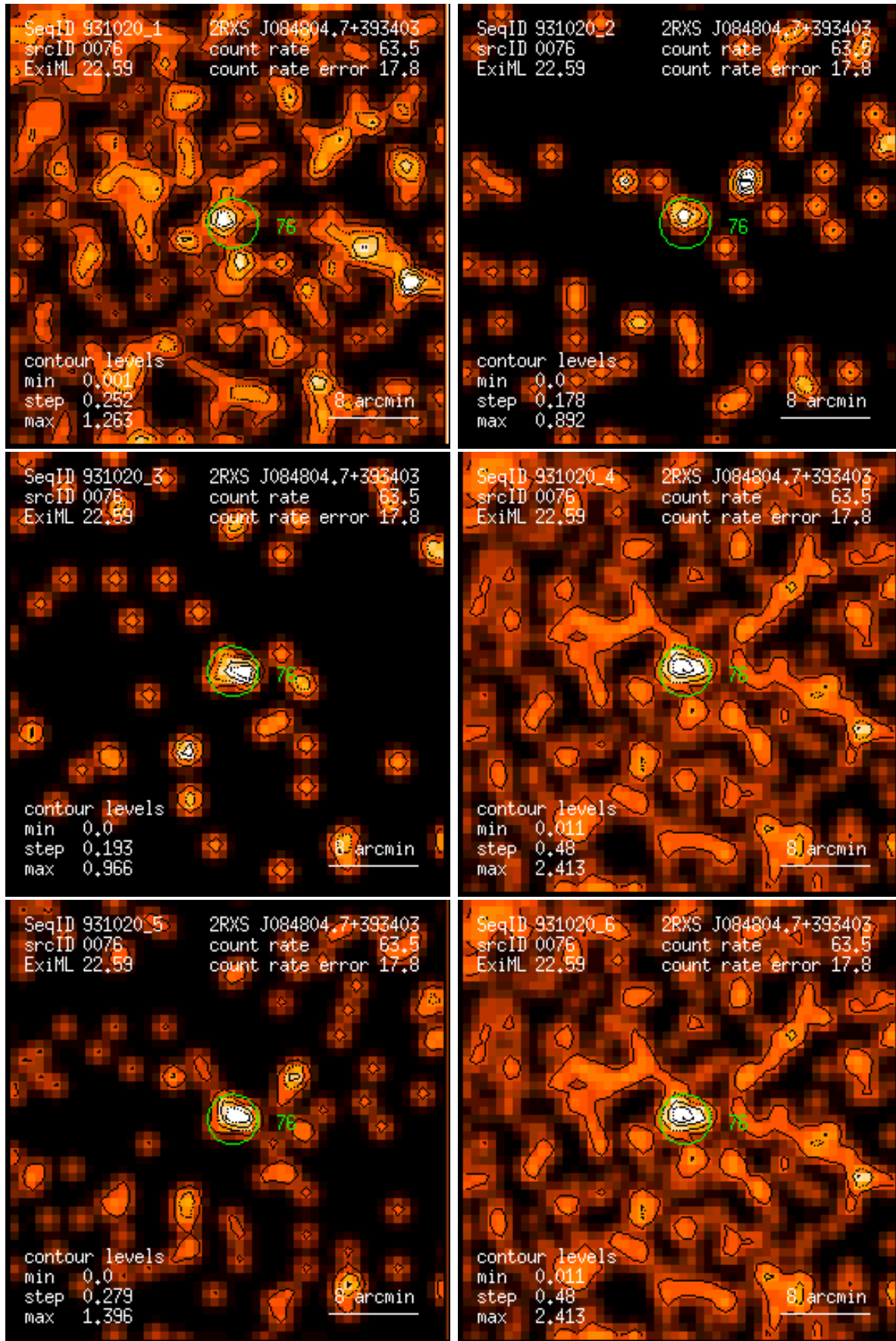
Figure 76: RASS 931020: detection 0076: band rate images, Gaussian filter: (1) PSPC channels 11 – 41, (2) 52 – 90, (3) 91 – 201, (4) 11 – 235, (5) 52 – 201, (6) 11 – 201. Broad band rates in counts/ks. Band rate contour levels in counts/ks/arcmin 2 .
