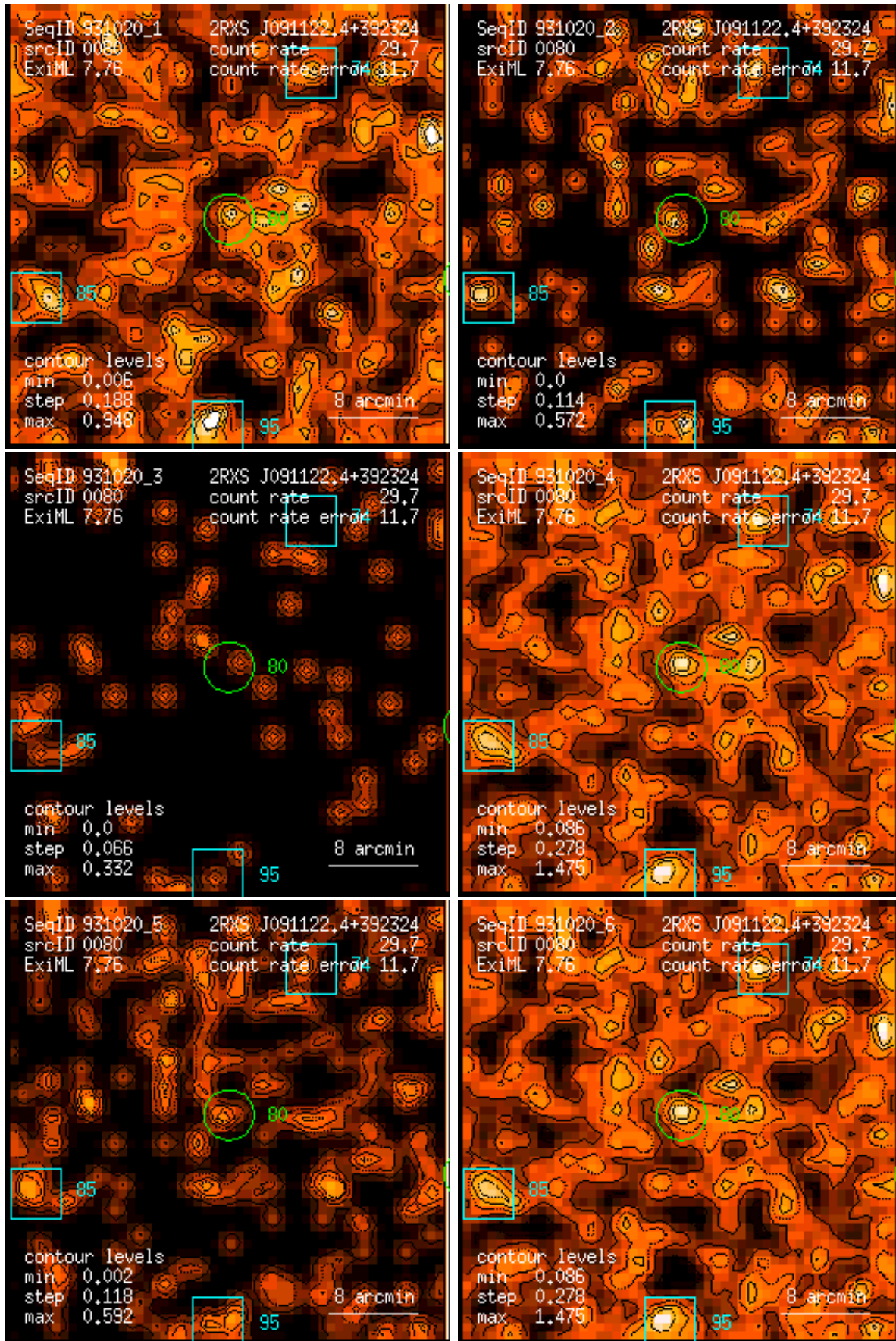
Figure 80: RASS 931020: detection 0080: band rate images, Gaussian filter: (1) PSPC channels 11 – 41, (2) 52 – 90, (3) 91 – 201, (4) 11 – 235, (5) 52 – 201, (6) 11 – 201. Broad band rates in counts/ks. Band rate contour levels in counts/ks/arcmin 2 .
