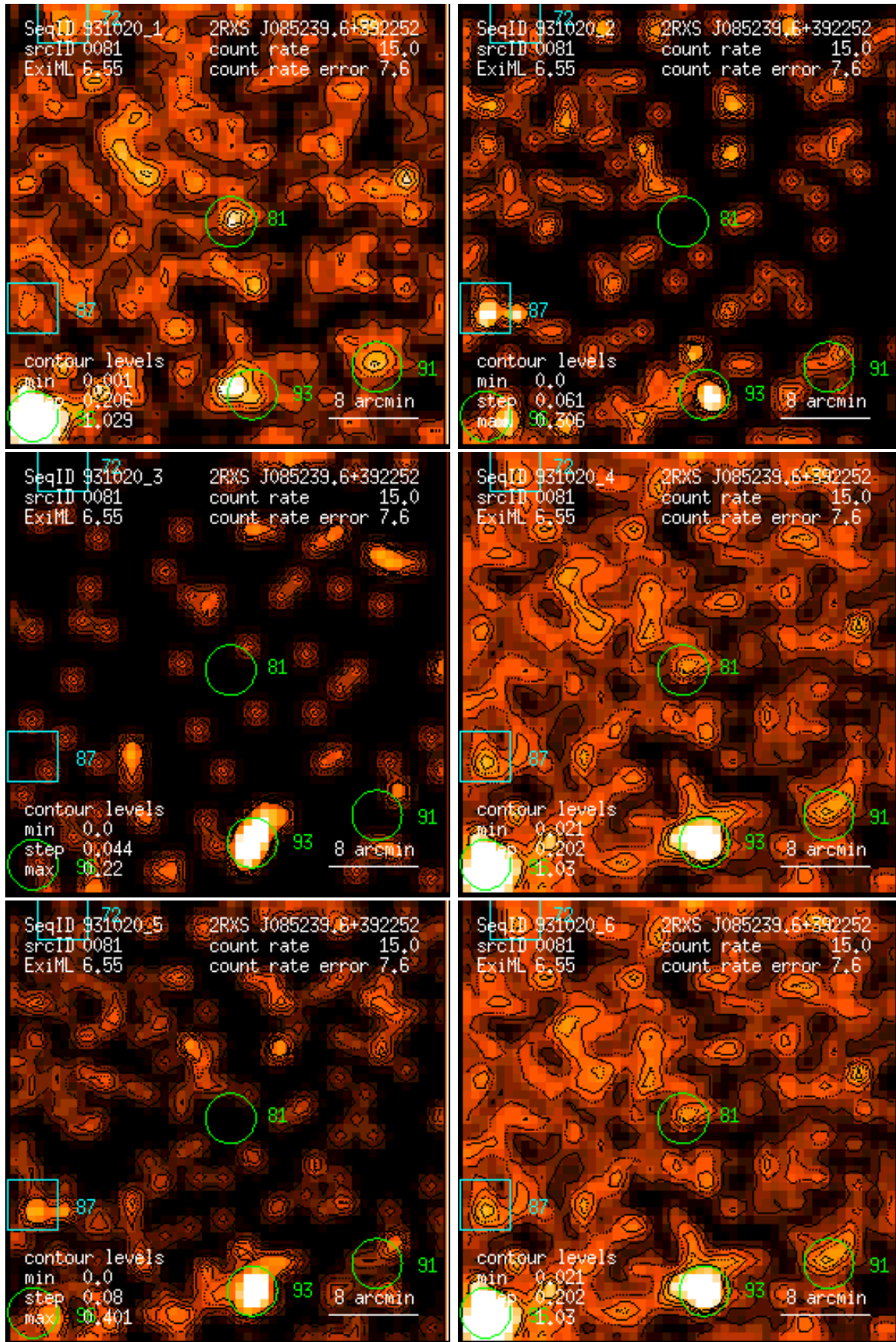
Figure 81: RASS 931020: detection 0081: band rate images, Gaussian filter: (1) PSPC channels 11 – 41, (2) 52 – 90, (3) 91 – 201, (4) 11 – 235, (5) 52 – 201, (6) 11 – 201. Broad band rates in counts/ks. Band rate contour levels in counts/ks/arcmin 2 .
