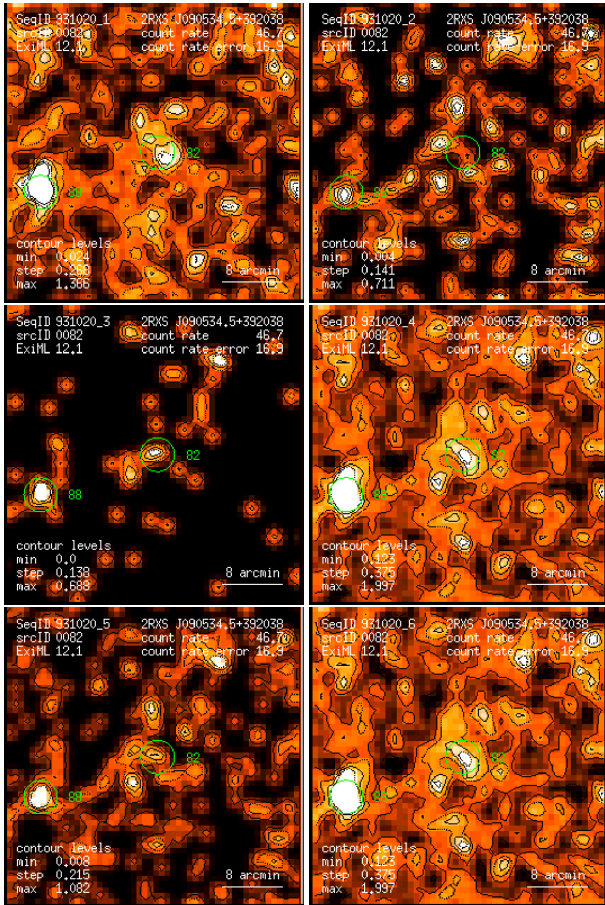
Figure 82: RASS 931020: detection 0082: band rate images, Gaussian filter: (1) PSPC channels 11 – 41, (2) 52 – 90, (3) 91 – 201, (4) 11 – 235, (5) 52 – 201, (6) 11 – 201. Broad band rates in counts/ks. Band rate contour levels in counts/ks/arcmin 2 .
